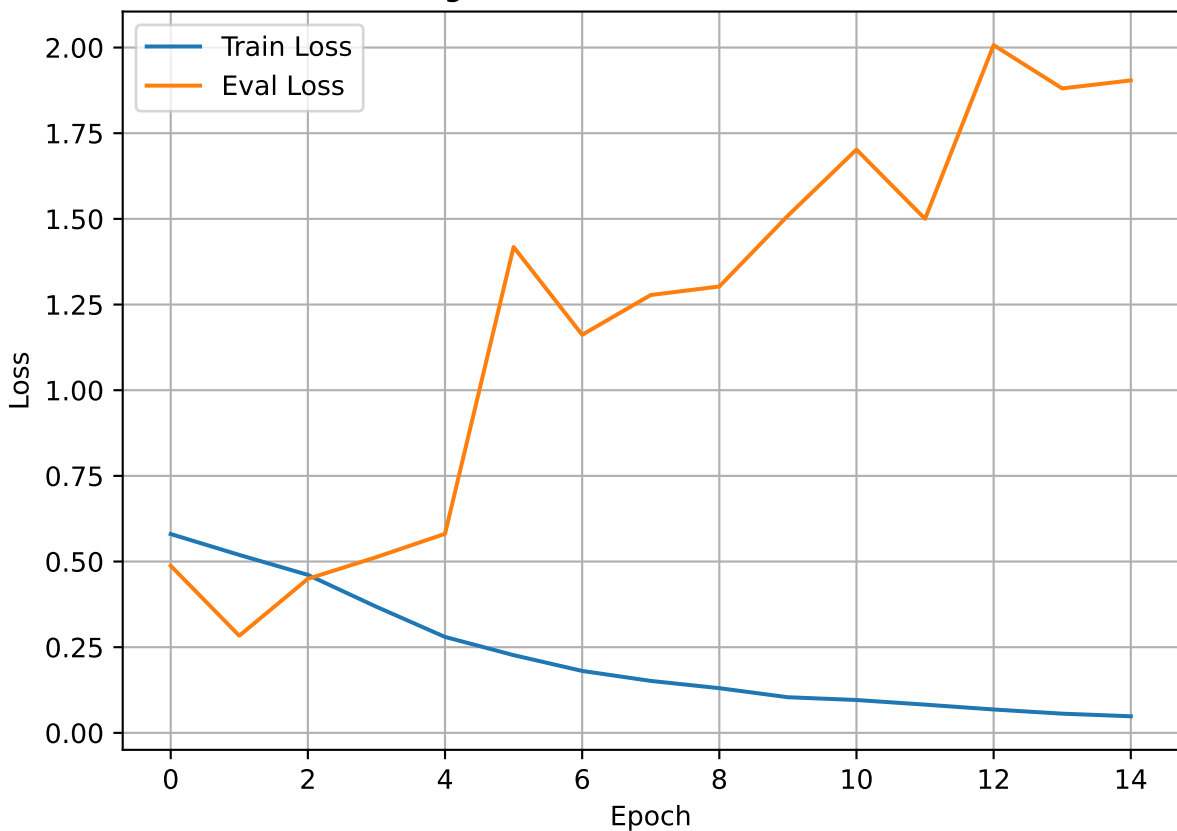
Training vs Evaluation Loss - CodeBERT
