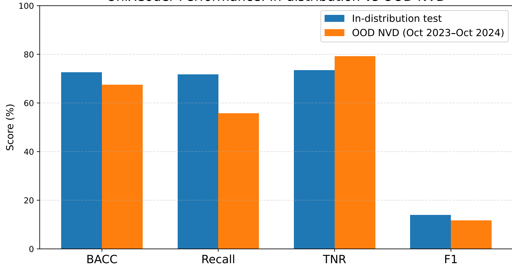
UniXCoder Performance: In-distribution vs OOD NVD
