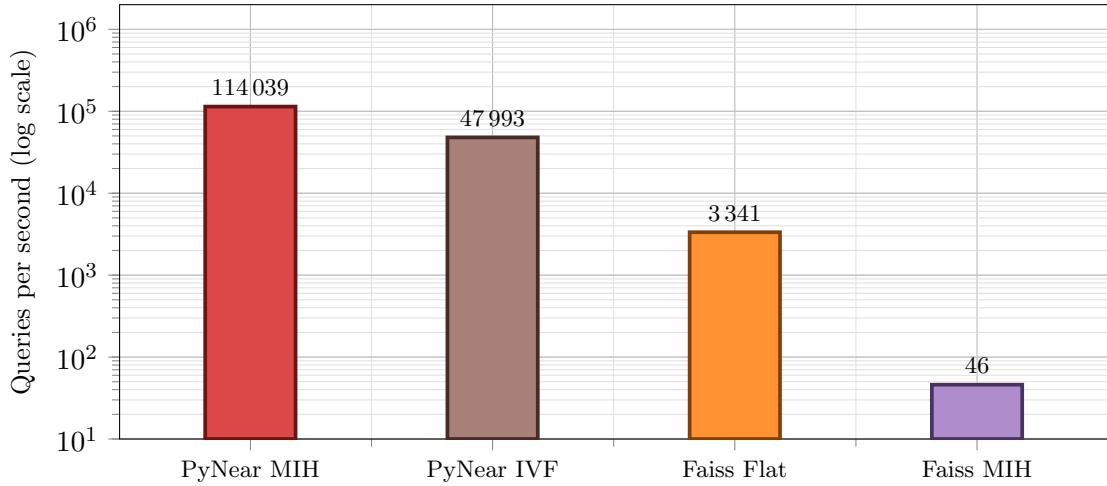
Figure 8: Throughput at 100% Recall@10 for 512-bit near-duplicate retrieval ( N = 10^6 , k = 10 , 24 threads; data of Table 3, log scale). PyNear MIHBinaryIndex sustains 34× the throughput of Faiss’s subprocess-isolated exact scan; Faiss’s own MIH implementation is \sim 2,500\times slower at this descriptor width.
