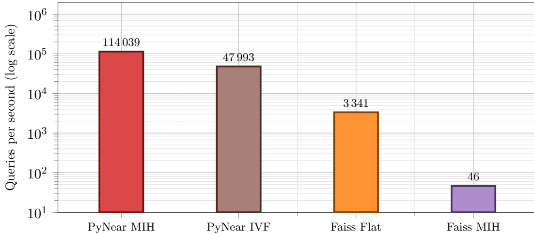
Figure 8: Throughput at 100% Recall@10 for 512-bit near-duplicate retrieval ( N = 10^6 , k = 10 , 24 threads; data of Table 3, log scale). PyNear MIHBinaryIndex sustains 34\times the throughput of Faiss’s subprocess-isolated exact scan; Faiss’s own MIH implementation is \sim 2,500\times slower at this descriptor width.
