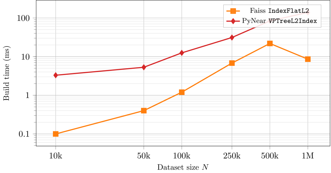
Figure 7: Exact-index build time (ms, log-log) vs. dataset size N , d = 32 . Faiss IndexFlatL2 requires no structural work (copy only), giving an O(N) lower bound (its non-monotonic 500k/1M points reflect allocator noise at sub-25-ms timescales). VPTreeL2Index follows an O(N \log N) curve, from 3.3 ms at N = 10\,000 to 139 ms at N = 10^6 — well within one-second build budgets for all tested sizes.
