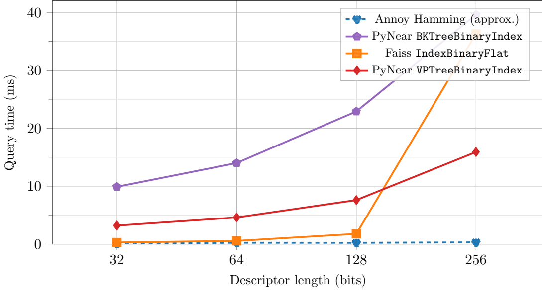
Figure 4: Mean query latency (ms) vs. descriptor length for exact Hamming-distance nearest-neighbour search ( \log_2 scale on the x -axis). Faiss’s flat binary index remains the fastest exact method at 32–128 bits, but at 256 bits VPTreeBinaryIndex (v2.4) is now 2.3\times faster (15.9 ms vs. 36.3 ms). Faiss is measured in-process here; see the OpenMP caveat in Section 2. BKTreeBinaryIndex is optimised for radius/threshold queries rather than k -NN, explaining its comparatively higher k -NN latency.
