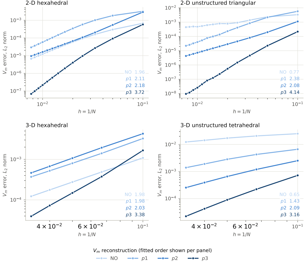
Figure 2: Spatial order of V_m for the four reconstruction levels on the diagonal, in 2-D ( N = 10 –130) and 3-D ( N = 10 –30), on structured and unstructured meshes. The number in each panel is the order fitted over that panel’s whole range. The four levels are an ordered scale, so they are drawn as one hue light to dark rather than as four categorical colours. Generated by figures/fig_orders.py from the raw errors_vs_N files.
