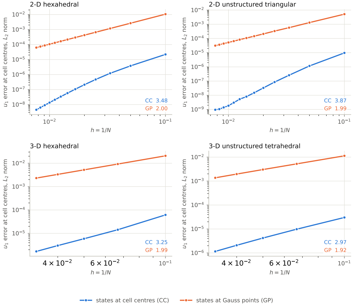
Figure 3: Error of the ionic state u_1 at cell centres, cellCentredReconstruct against gaussPointODE , with the (p3, \cdot, p3) triad. The Gauss-point mode is pinned at order two in every panel; the cell-centred mode follows the scheme. Generated by figures/fig_orders.py .
