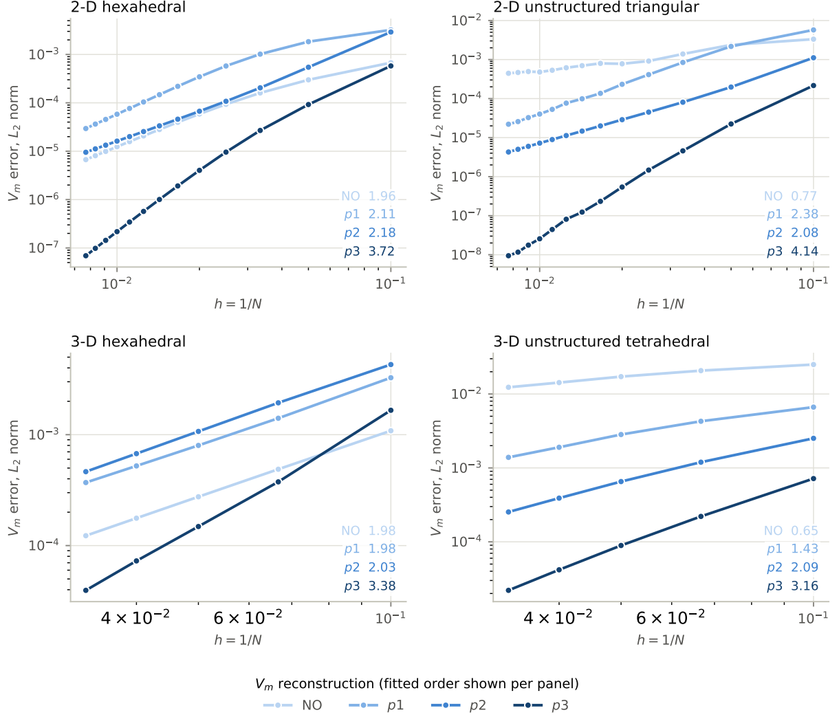
Figure 2: Spatial order of V_m for the four reconstruction levels on the diagonal, in 2-D ( N = 10 – 130 ) and 3-D ( N = 10 – 30 ), on structured and unstructured meshes. The number in each panel is the order fitted over that panel's whole range. The four levels are an ordered scale, so they are drawn as one hue light to dark rather than as four categorical colours. Generated by figures/fig_orders.py from the raw errors_vs_N files.
