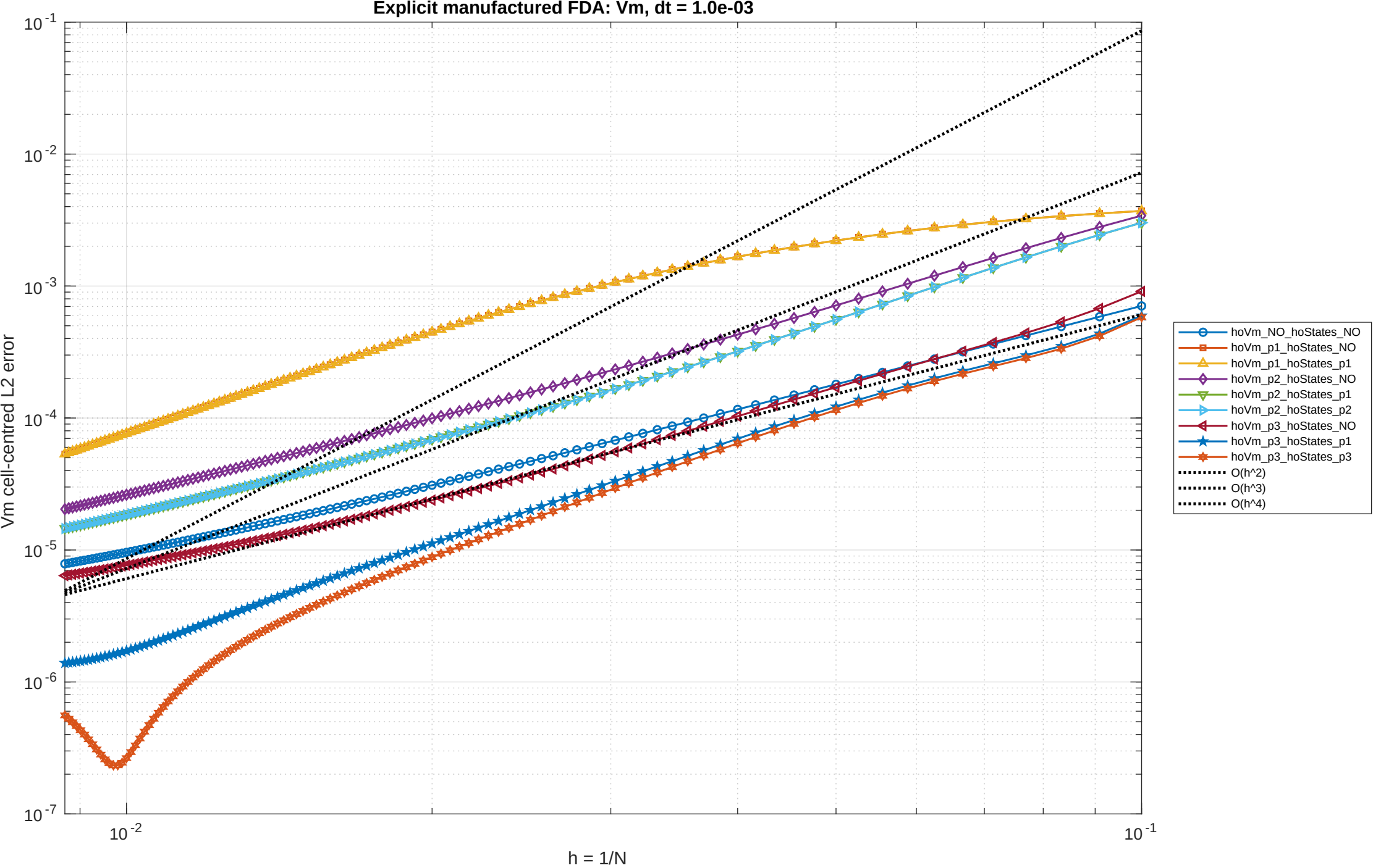
Explicit manufactured FDA: Vm, dt = 1.0e-03
