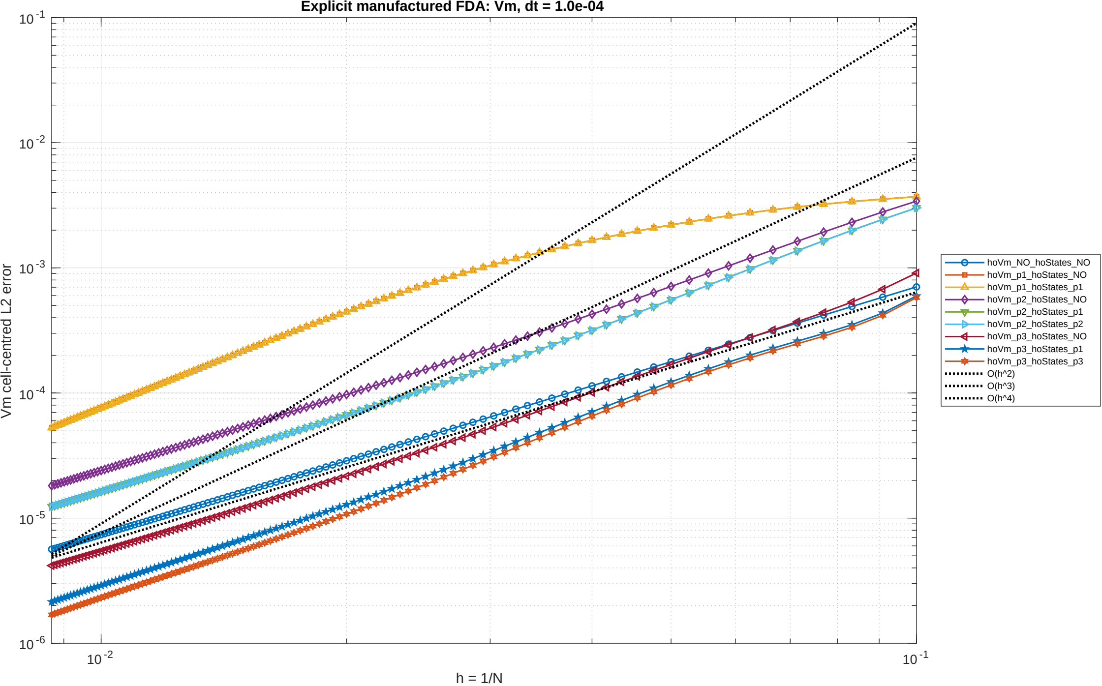
Explicit manufactured FDA: Vm, dt = 1.0e-04
