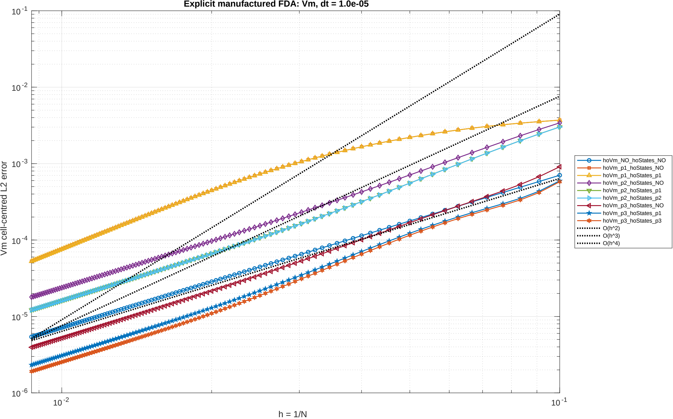
Explicit manufactured FDA: Vm, dt = 1.0e-05
