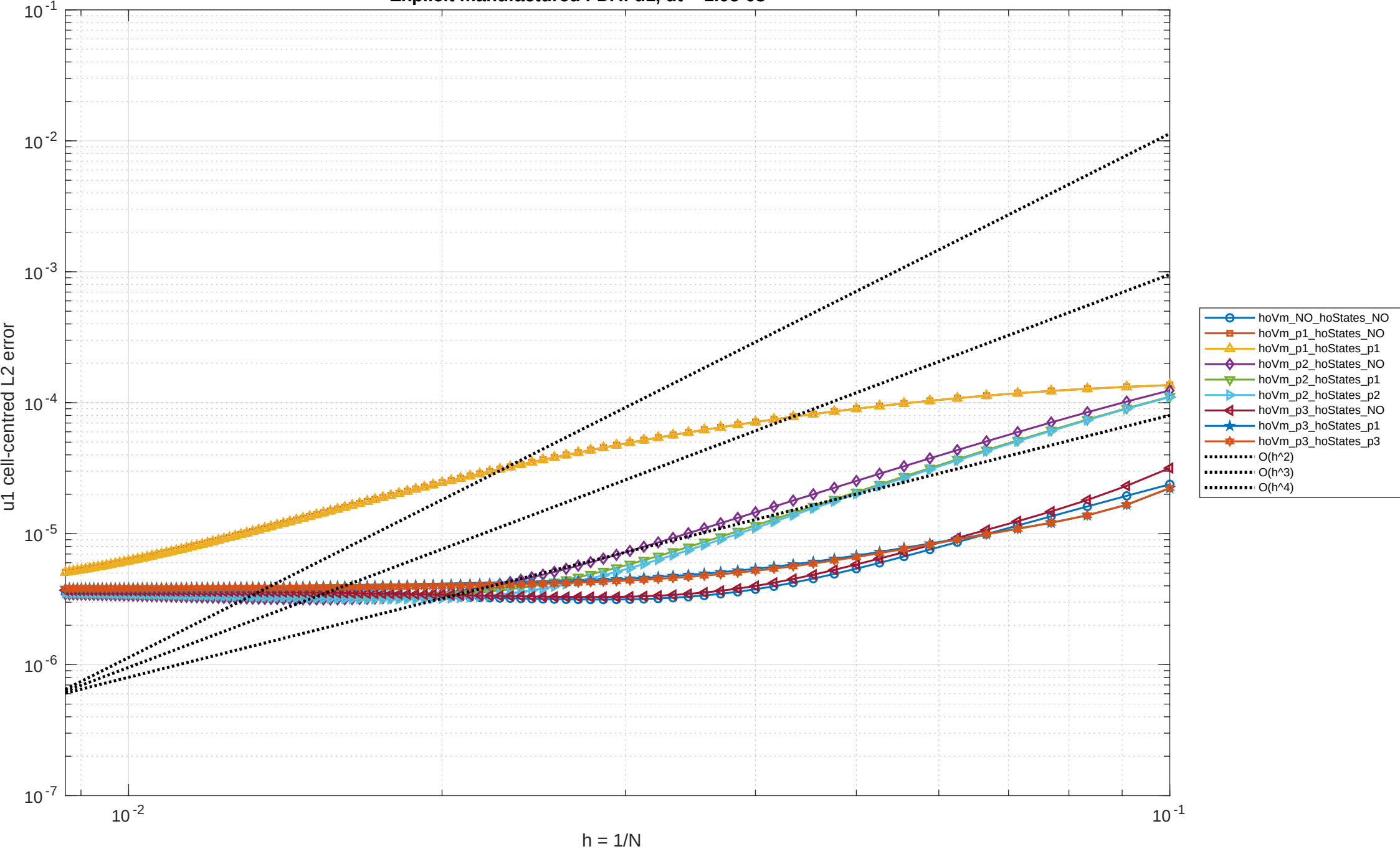
Explicit manufactured FDA: u1, dt = 1.0e-03
