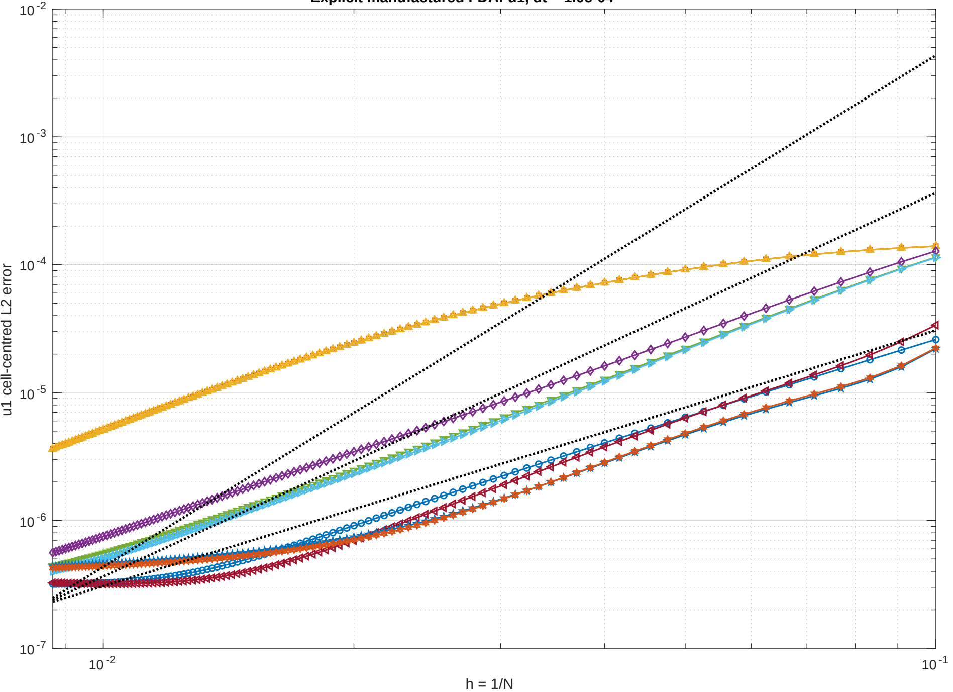
Explicit manufactured FDA: u1, dt = 1.0e-04
