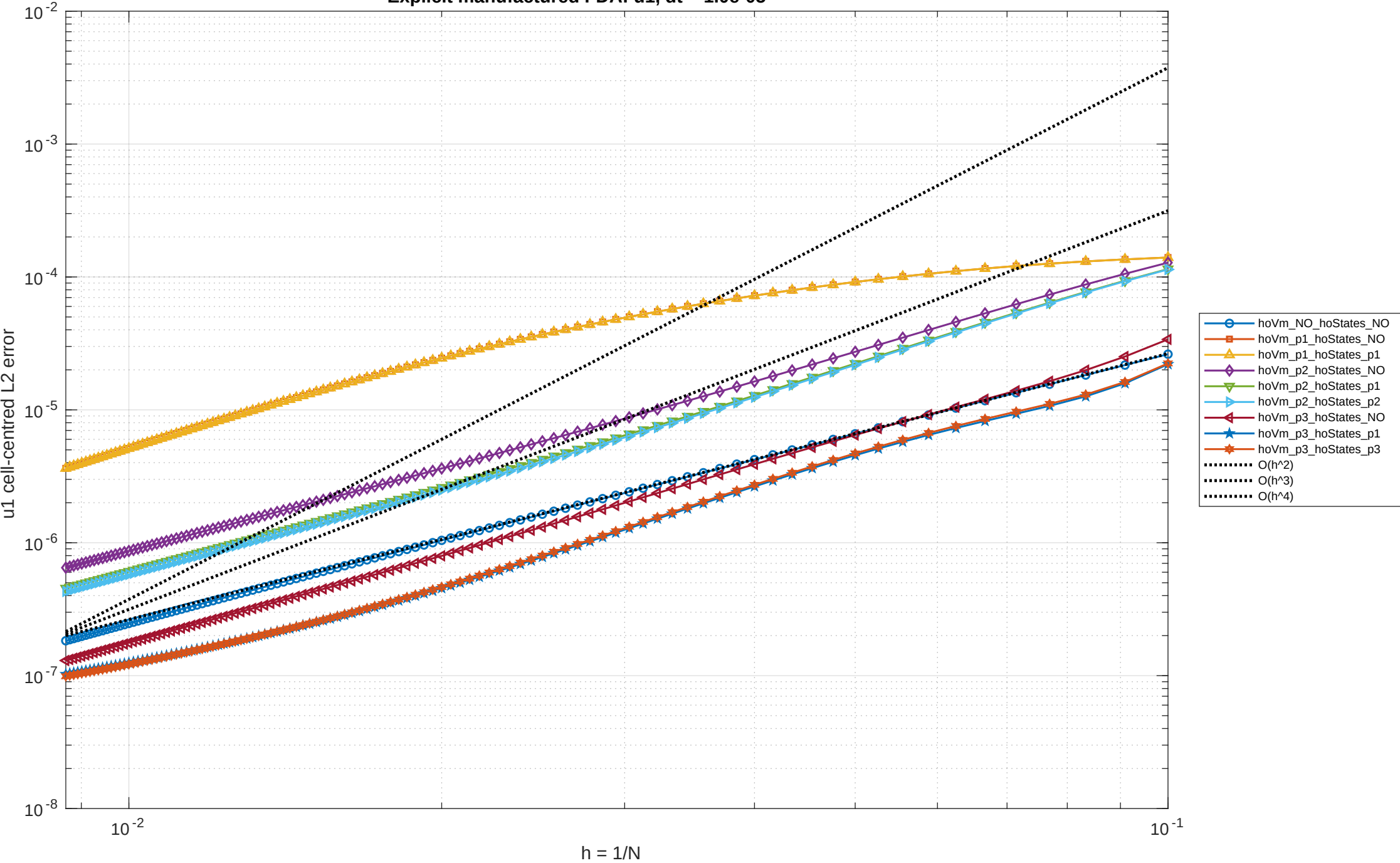
Explicit manufactured FDA: u1, dt = 1.0e-05
