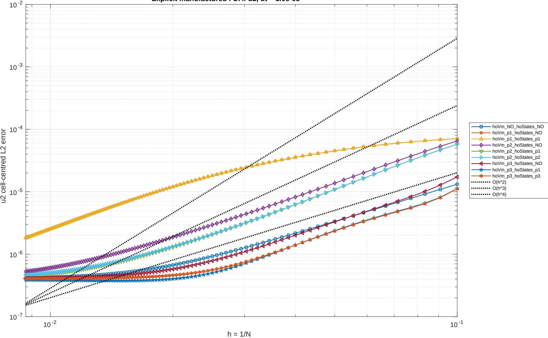
Explicit manufactured FDA: u2, dt = 1.0e-05
