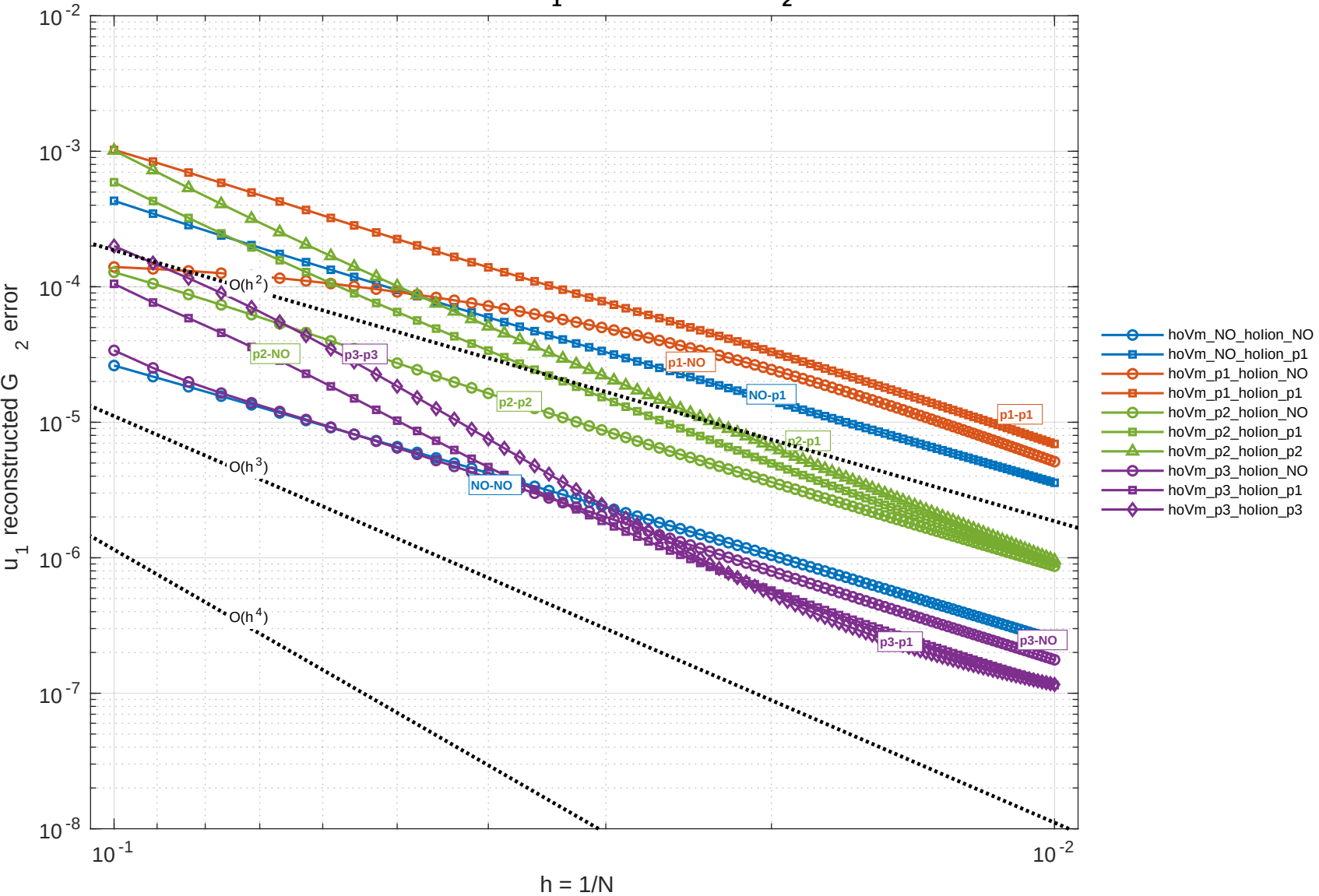
Explicit manufactured FDA: 2D, u_1 reconstructed G_2 error, dt = 1.0e-05
