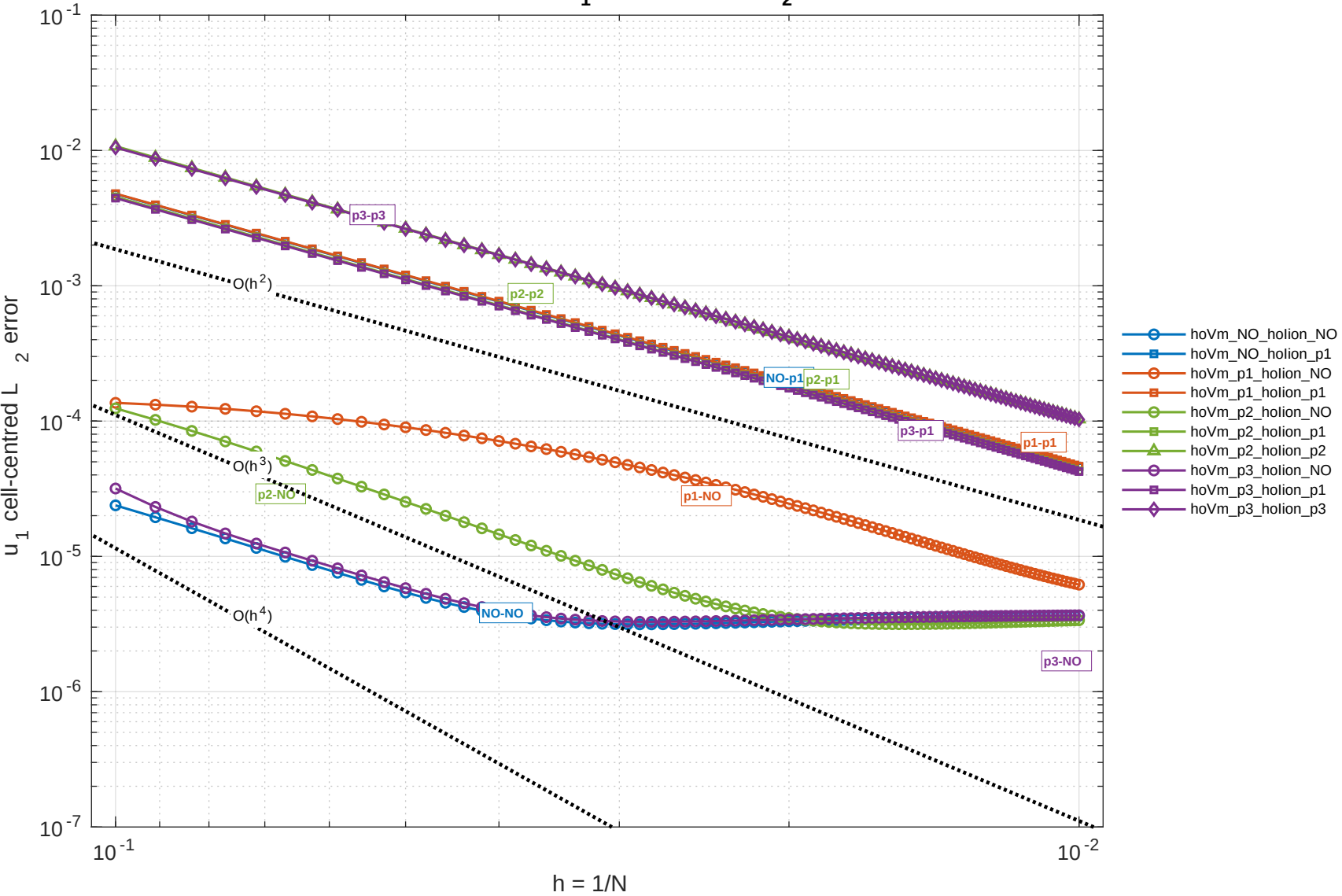
Explicit manufactured FDA: 2D, u_1 cell-centred L 2 error, dt = 1.0e-03
