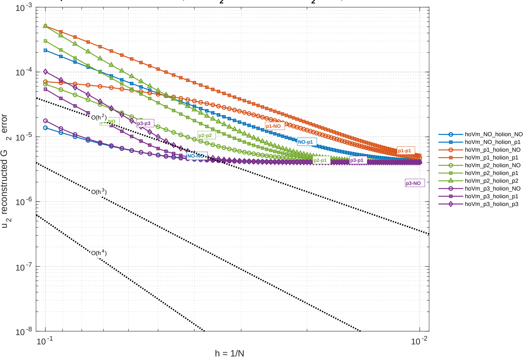
Explicit manufactured FDA: 2D, u_2 reconstructed G_2 error, dt = 1.0e-04
