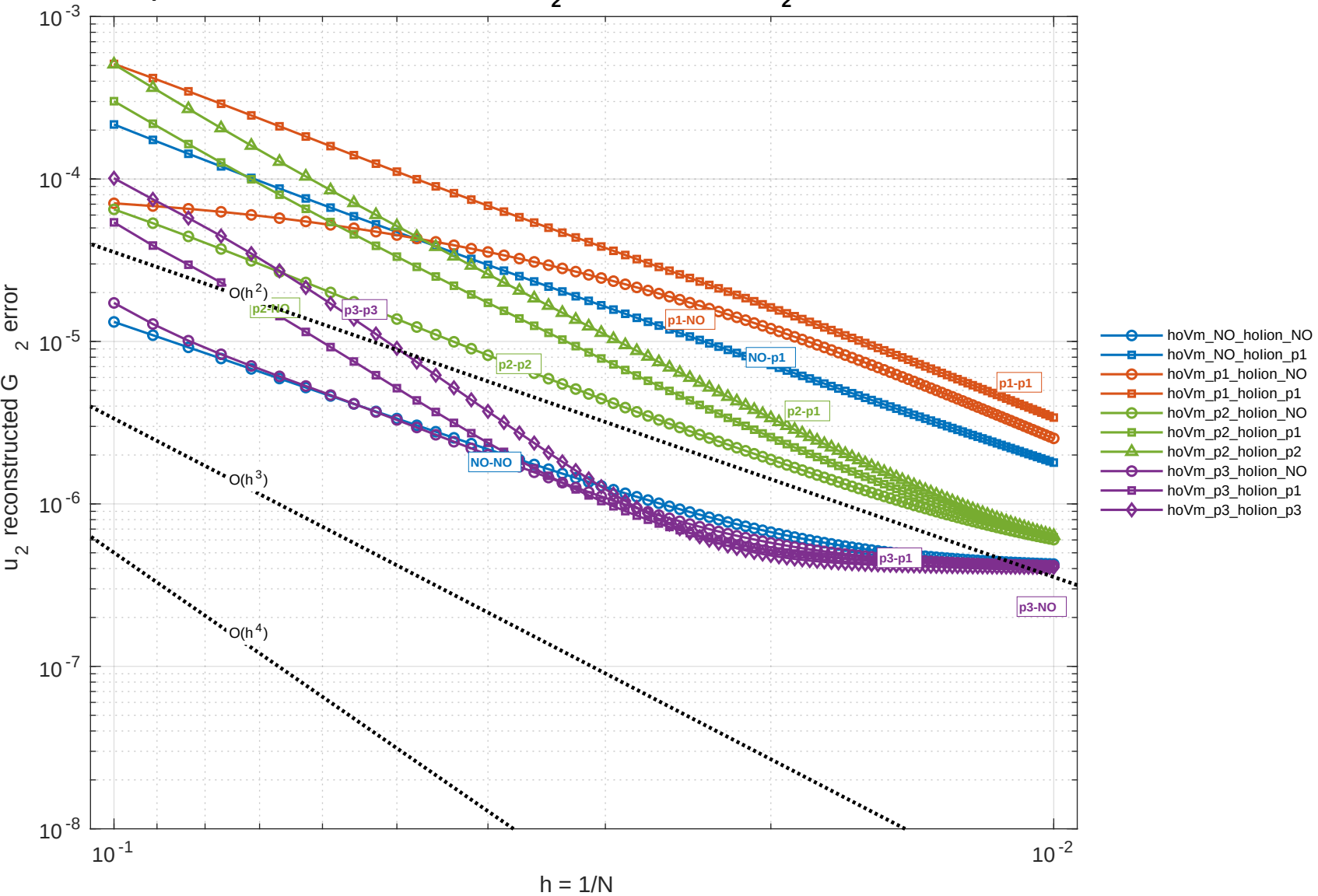
Explicit manufactured FDA: 2D, u_2 reconstructed G_2 error, dt = 1.0e-05
