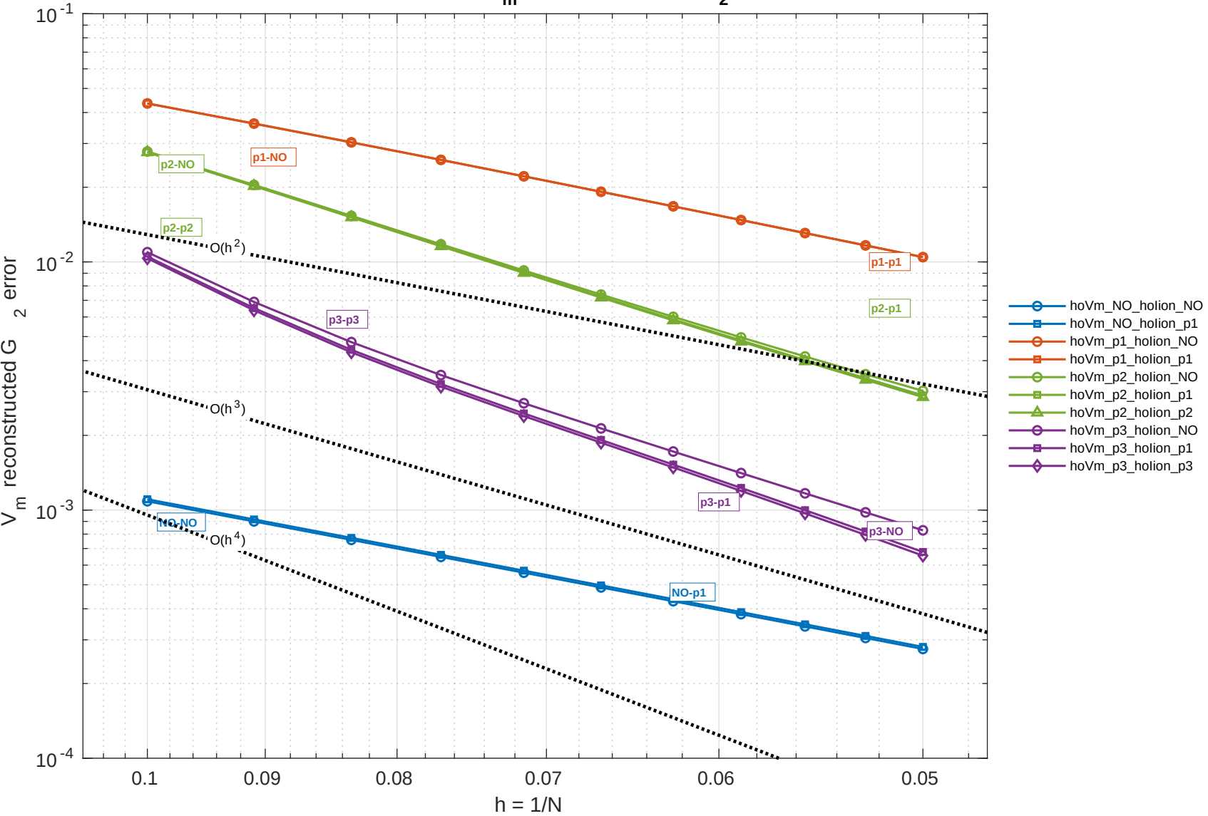
Explicit manufactured FDA: 3D, V_m reconstructed G_2 error, dt = 1.0e-04
