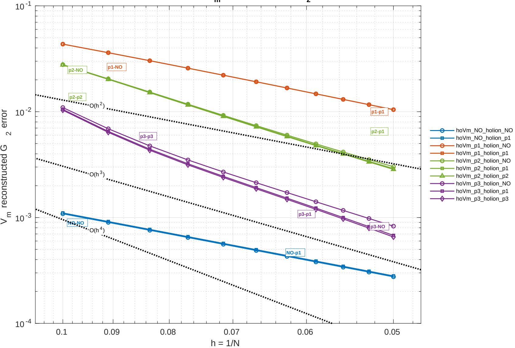
Explicit manufactured FDA: 3D, V_m reconstructed G_2 error, dt = 1.0e-05
