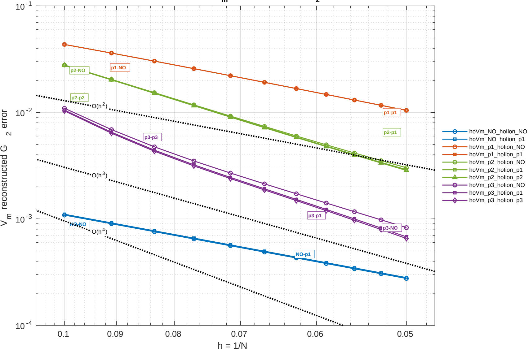
Explicit manufactured FDA: 3D, V m reconstructed G 2 error, dt = 1.0e-06
