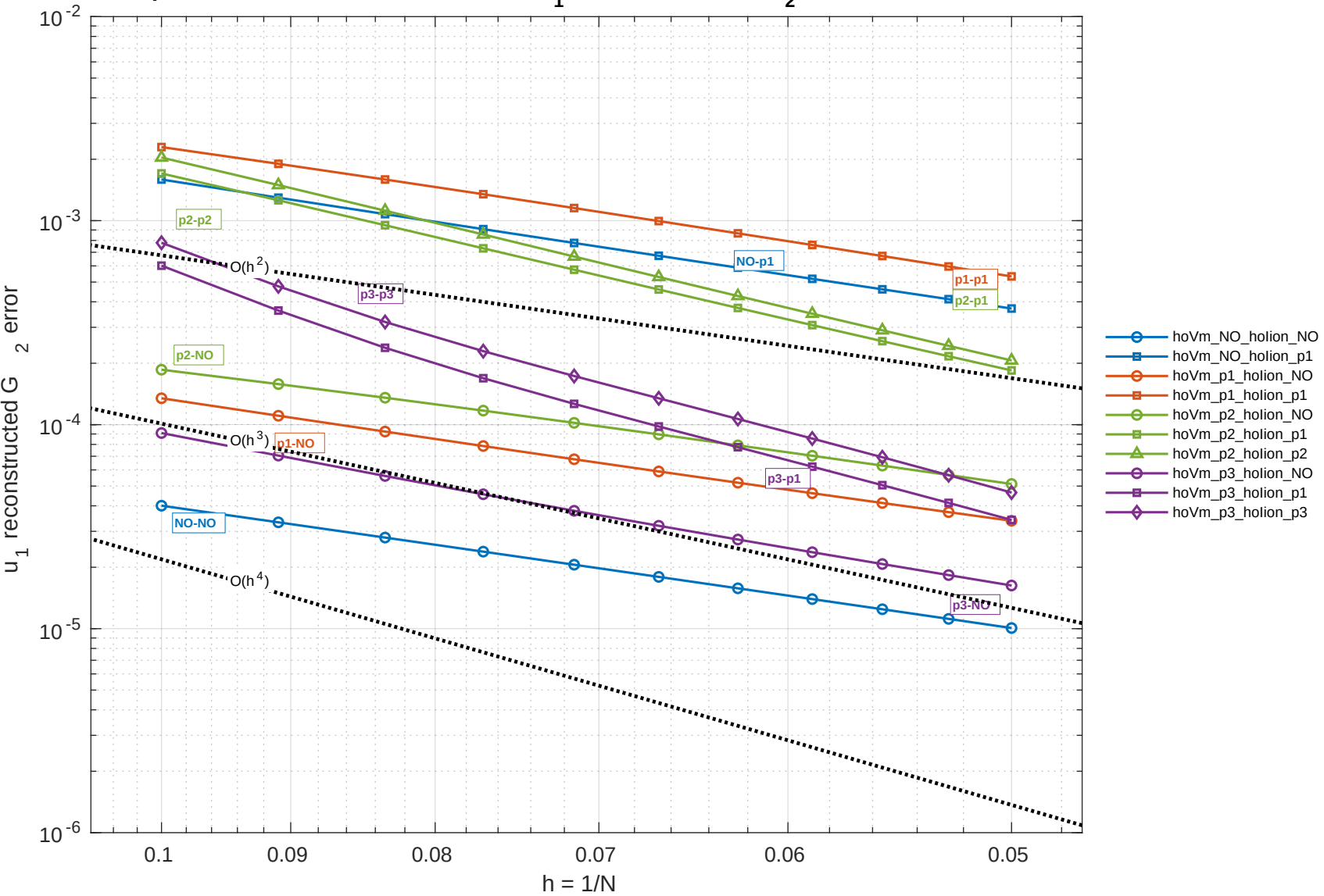
Explicit manufactured FDA: 3D, u_1 reconstructed G_2 error, dt = 1.0e-04
