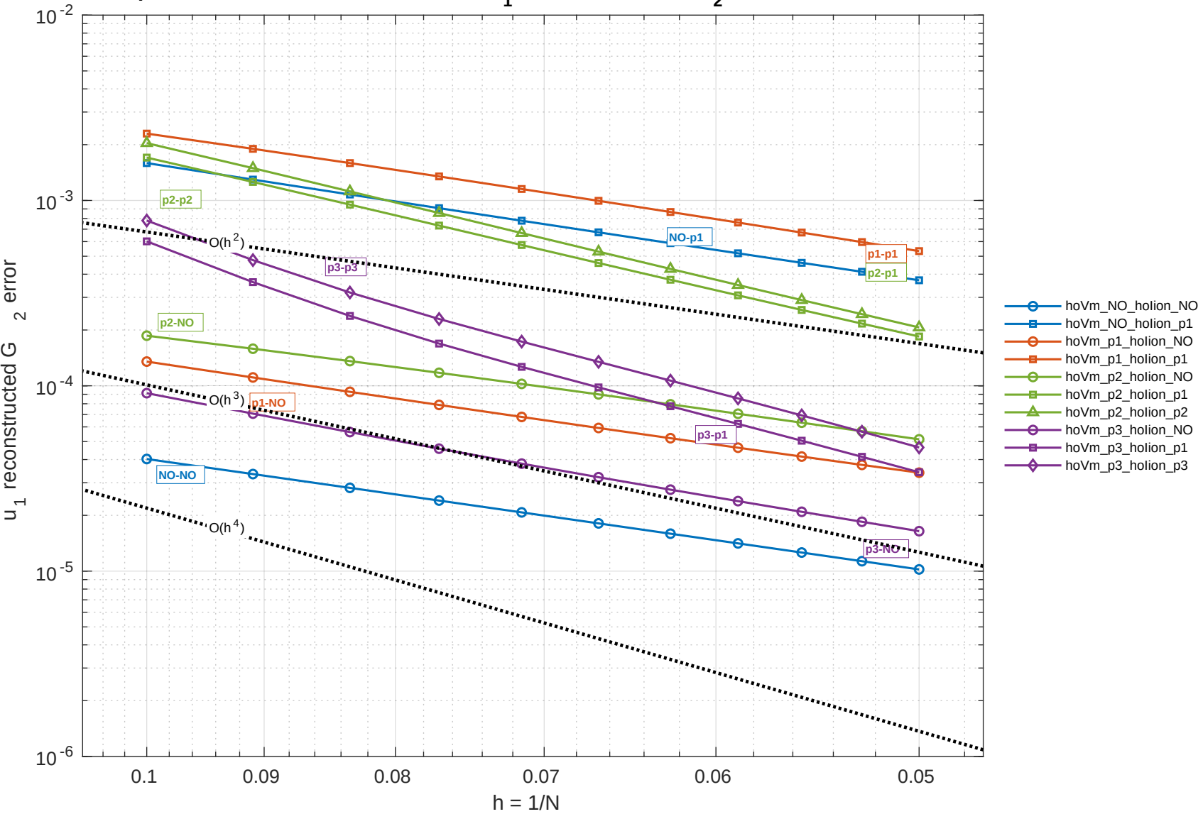
Explicit manufactured FDA: 3D, u_1 reconstructed G_2 error, dt = 1.0e-05
