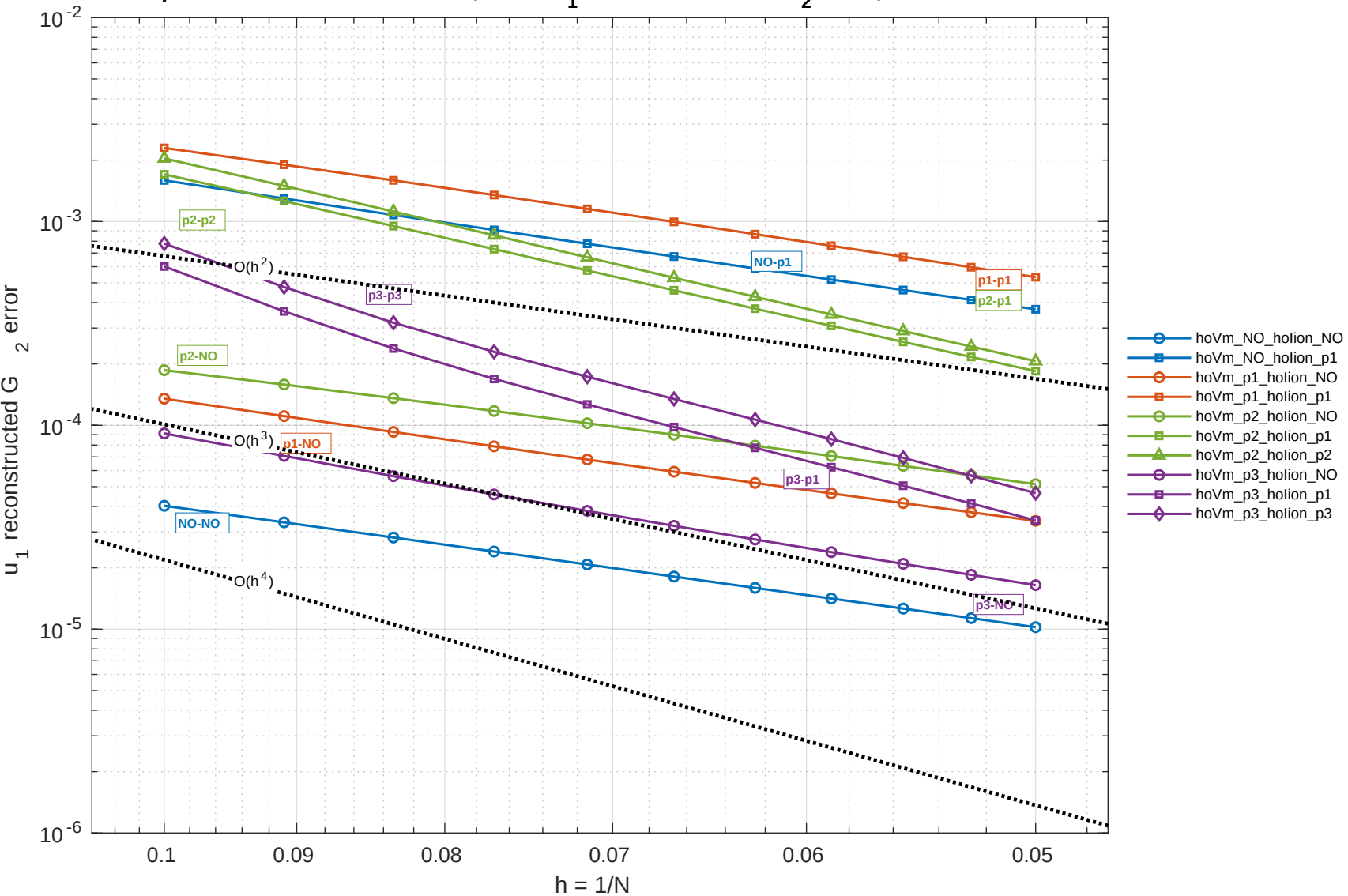
Explicit manufactured FDA: 3D, u_1 reconstructed G_2 error, dt = 1.0e-06
