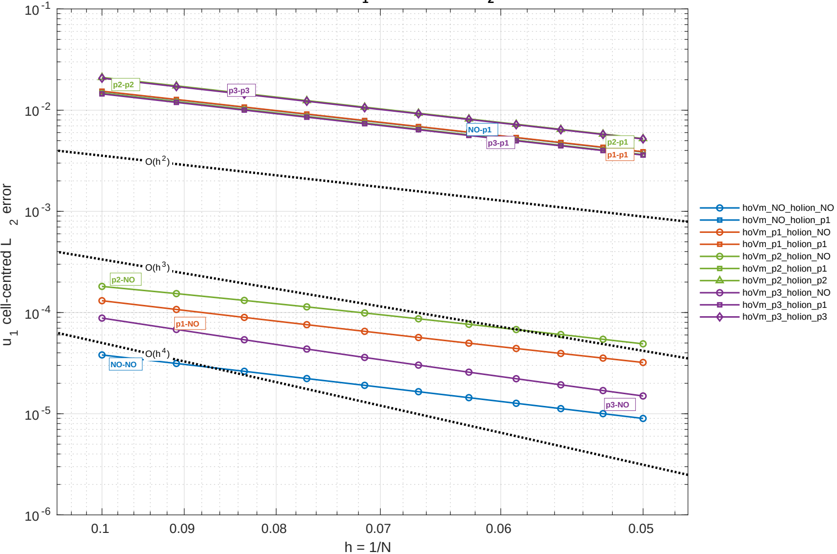
Explicit manufactured FDA: 3D, u_1 cell-centred L_2 error, dt = 1.0e-03
