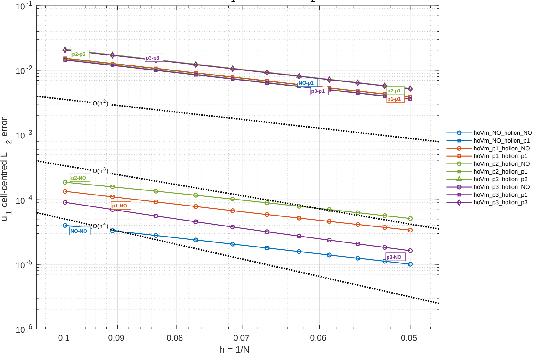
Explicit manufactured FDA: 3D, u_1 cell-centred L_2 error, dt = 1.0e-04
