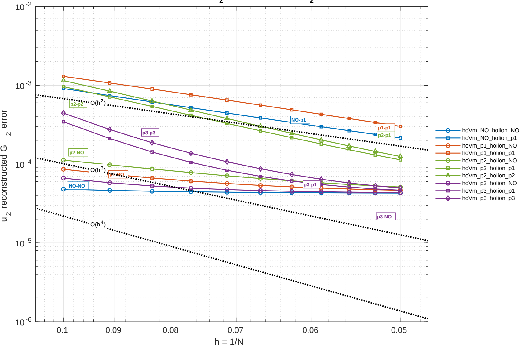
Explicit manufactured FDA: 3D, u_2 reconstructed G_2 error, dt = 1.0e-03
