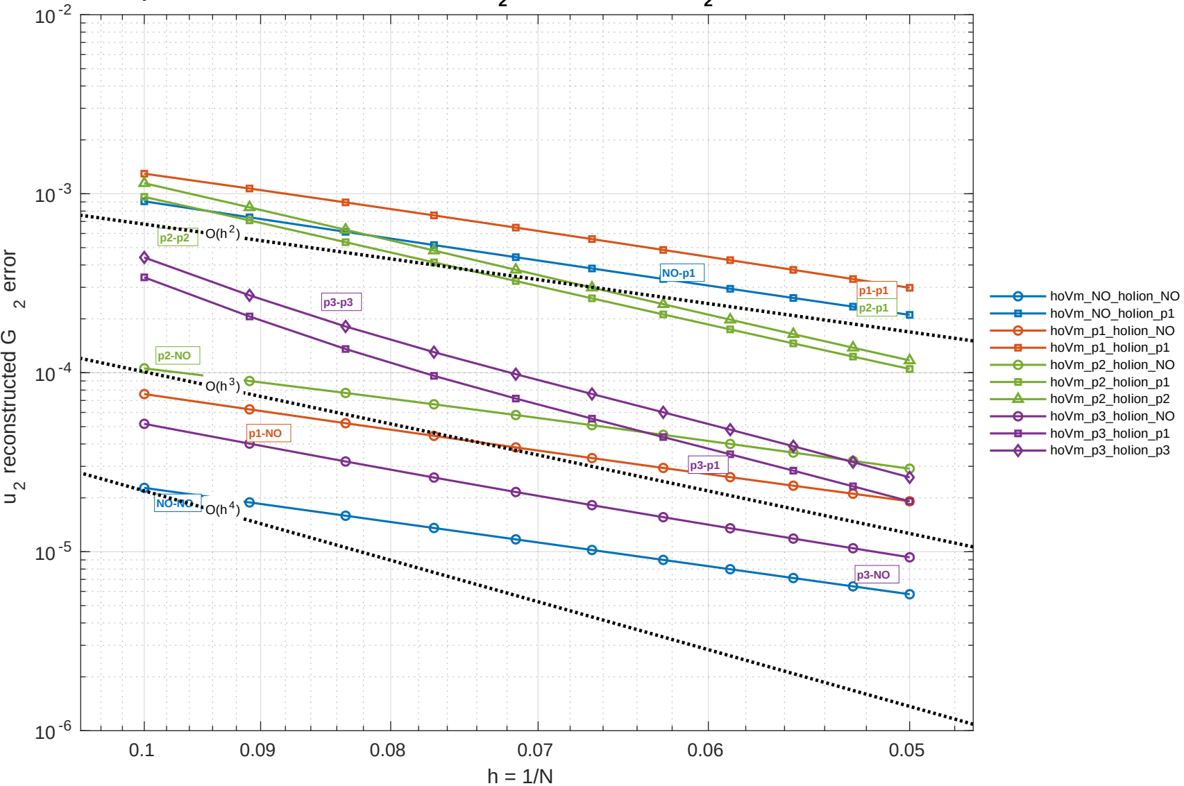
Explicit manufactured FDA: 3D, u_2 reconstructed G_2 error, dt = 1.0e-05
