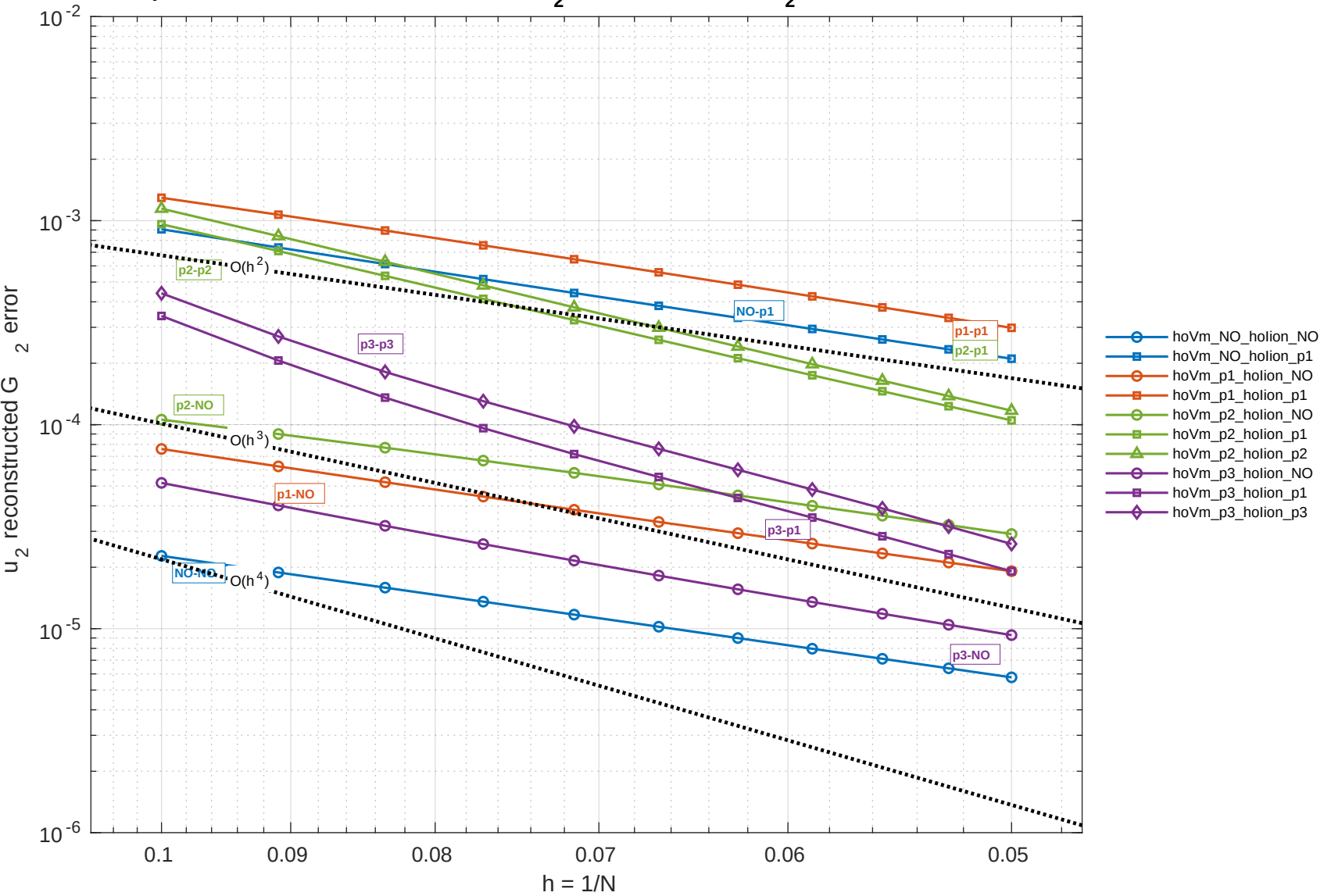
Explicit manufactured FDA: 3D, u_2 reconstructed G_2 error, dt = 1.0e-06
