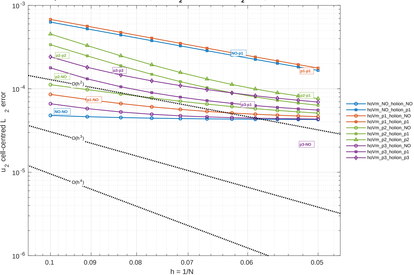
Explicit manufactured FDA: 3D, u_2 cell-centred L_2 error, dt = 1.0e-03
