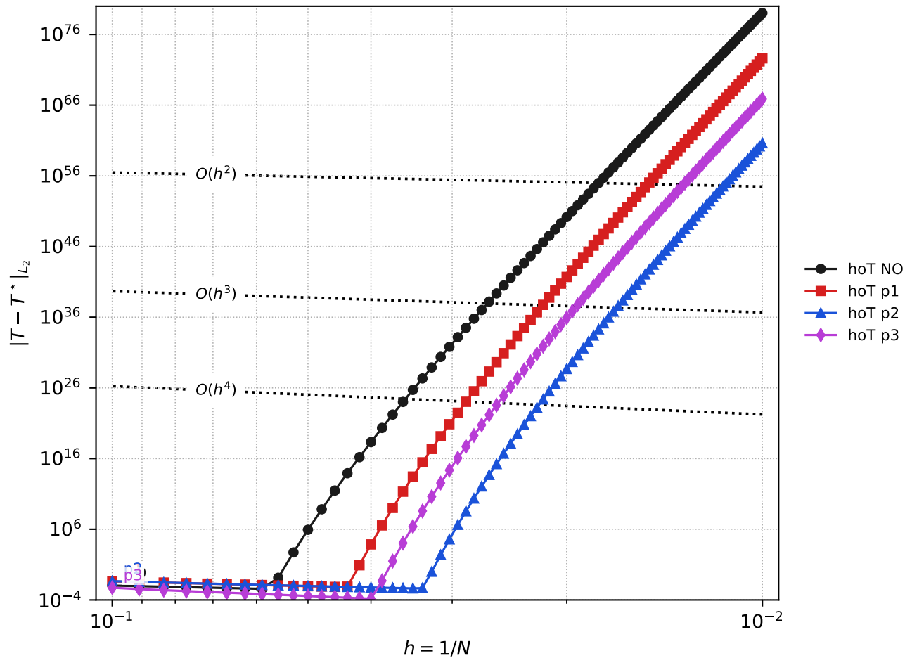
Explicit heat equation, 2D, dt = 0.001
