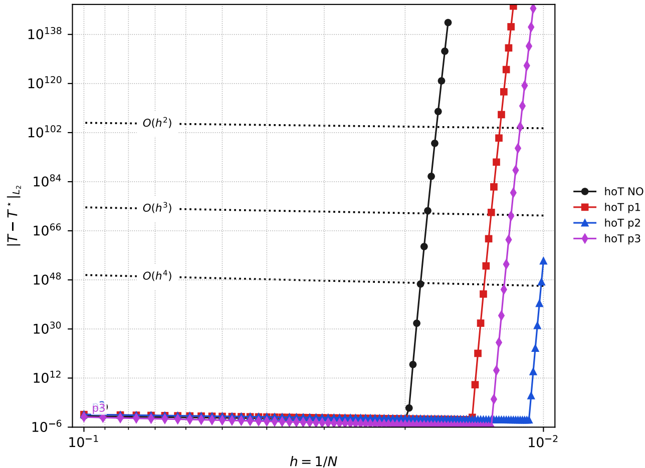
Explicit heat equation, 2D, dt = 0.0001
