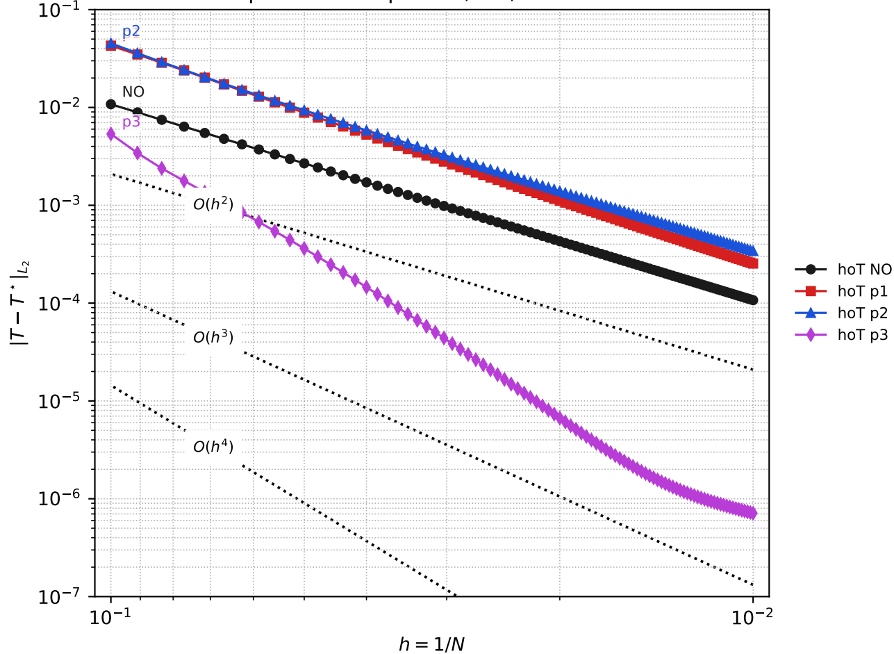
Explicit heat equation, 2D, dt = 1e-06
