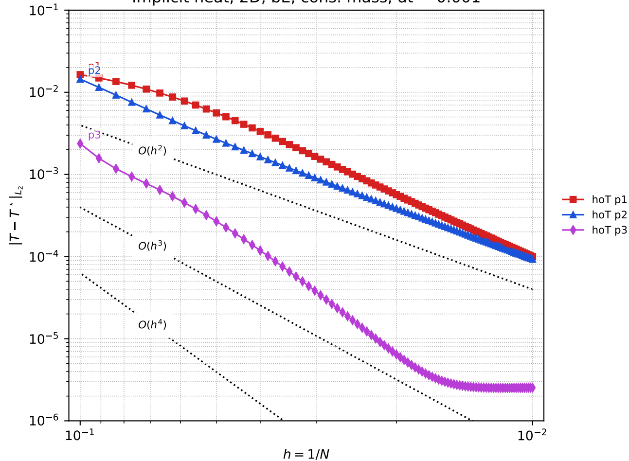
Implicit heat, 2D, bE, cons. mass, dt = 0.001
