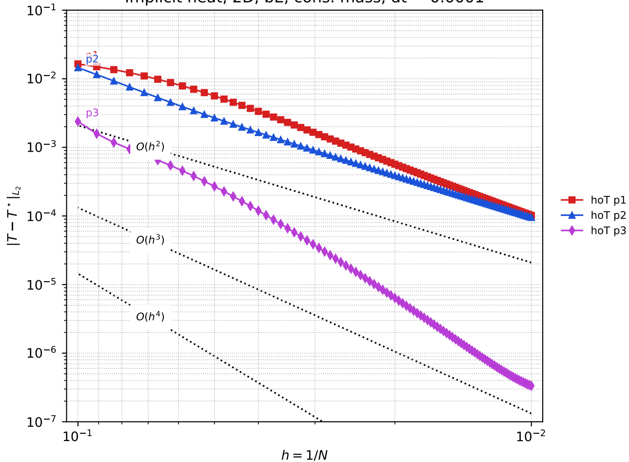
Implicit heat, 2D, bE, cons. mass, dt = 0.0001
