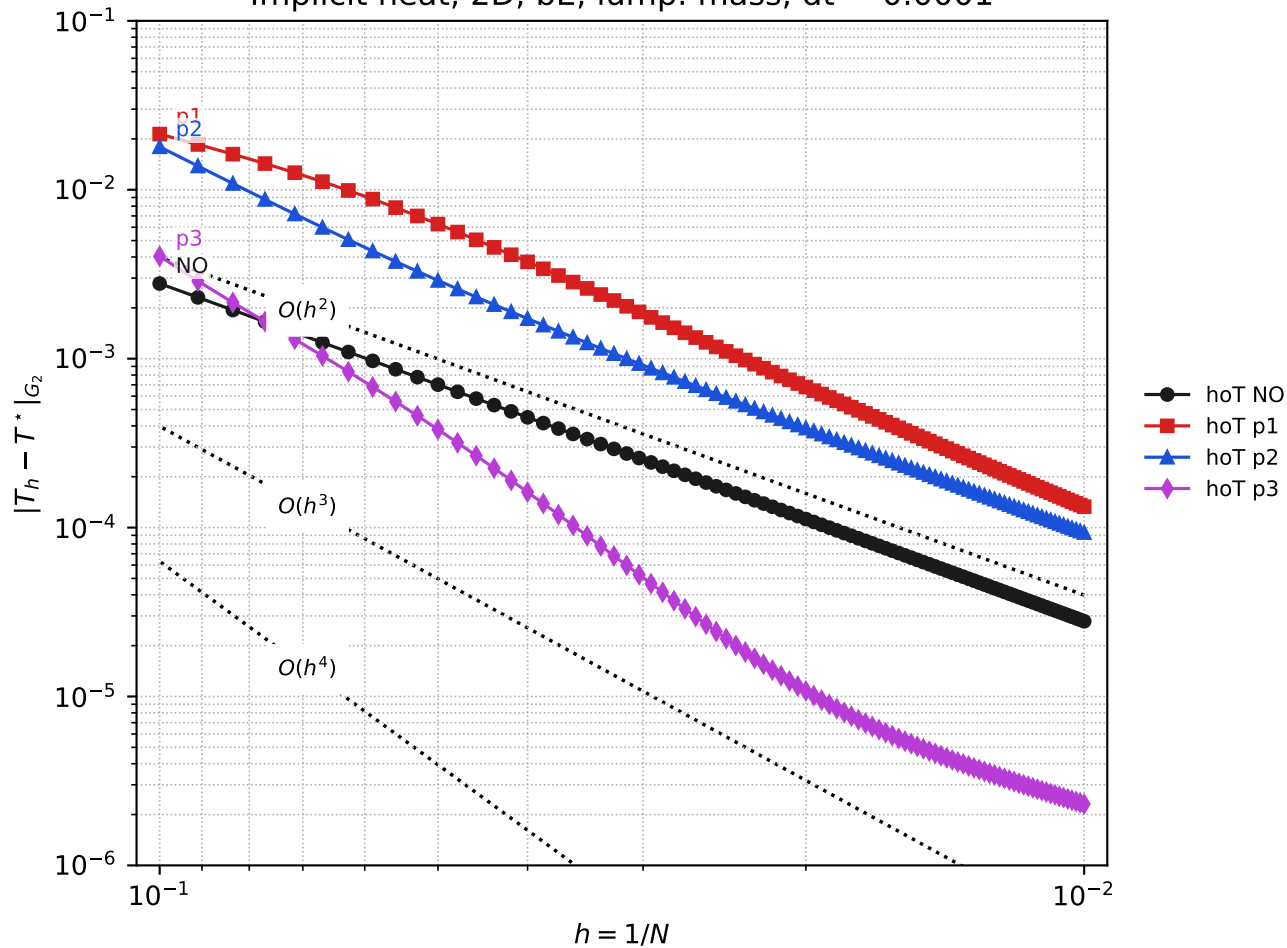
Implicit heat, 2D, bE, lump. mass, dt = 0.0001
