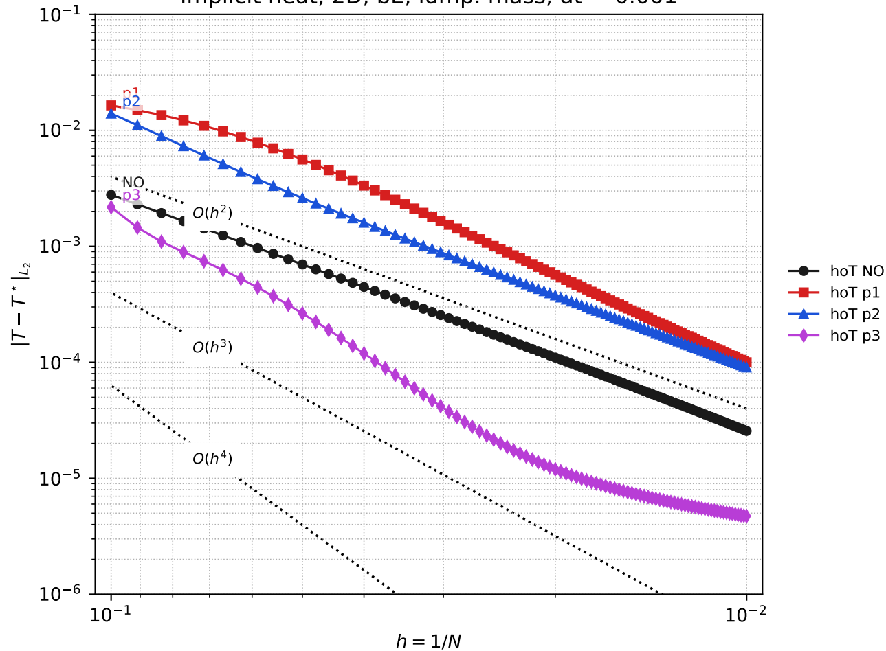
Implicit heat, 2D, bE, lump. mass, dt = 0.001
