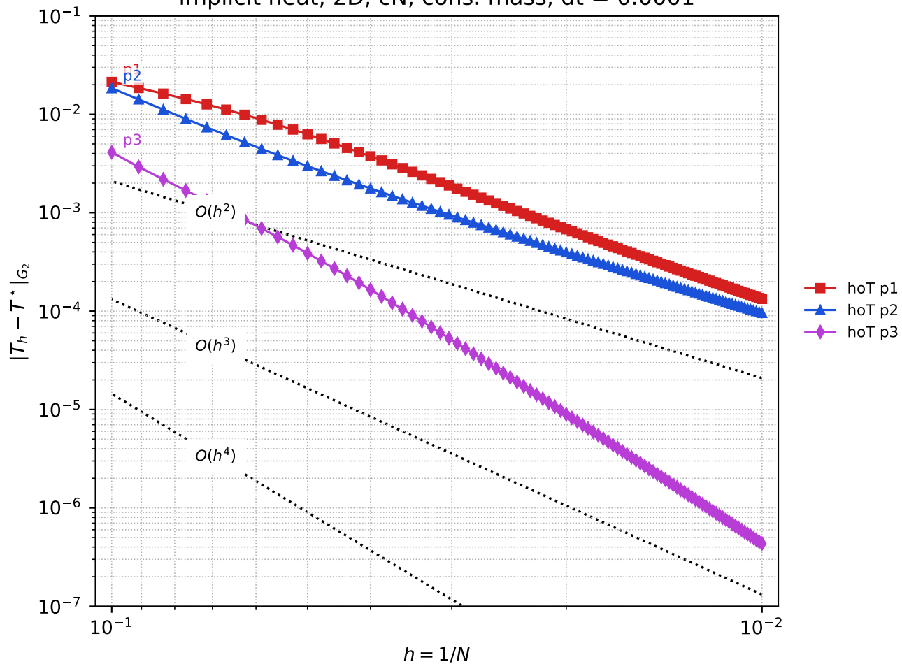
Implicit heat, 2D, cN, cons. mass, dt = 0.0001
