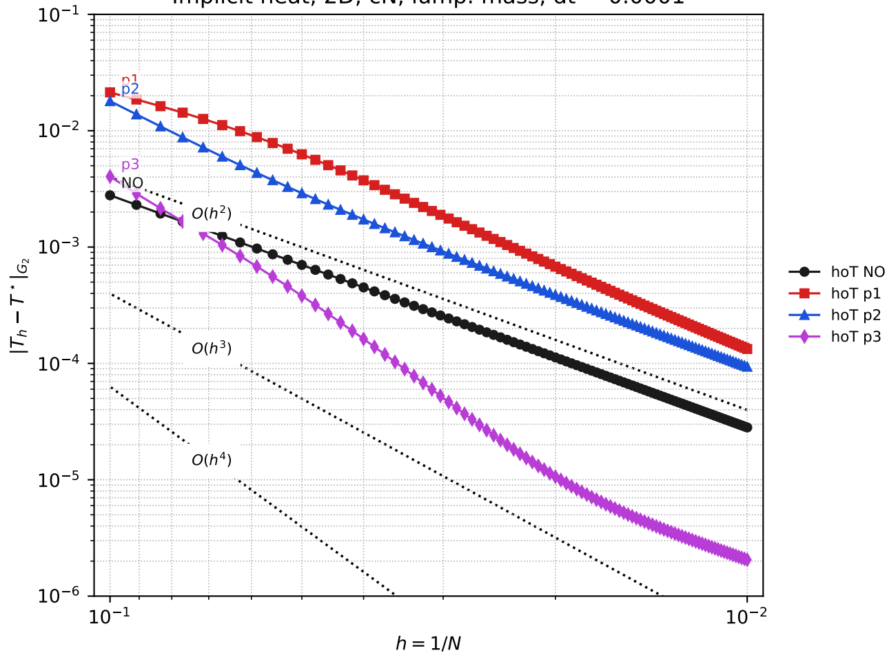
Implicit heat, 2D, cN, lump. mass, dt = 0.0001
