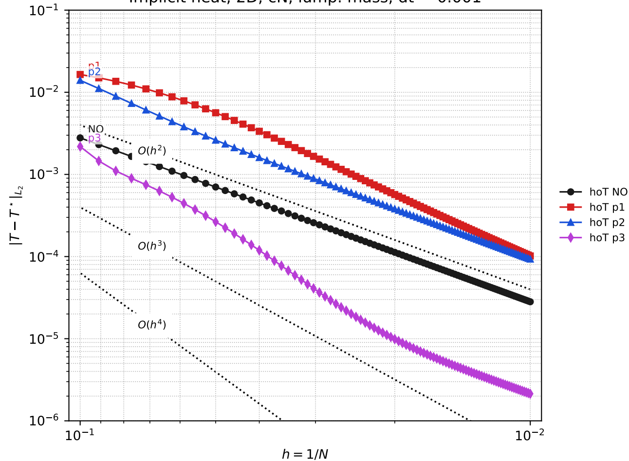
Implicit heat, 2D, cN, lump. mass, dt = 0.001
