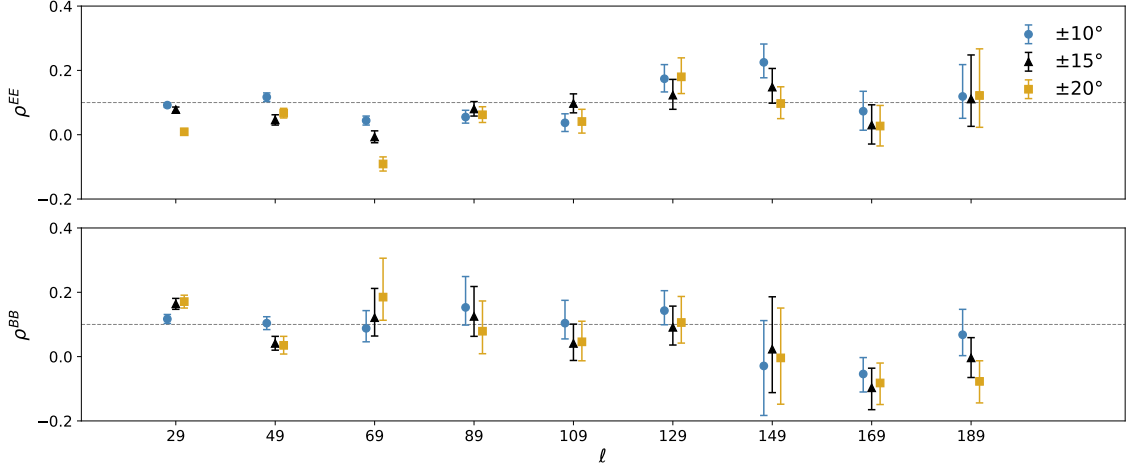
Figure 8: Synchrotron-dust spatial correlation \rho for E-modes (top panel) and B-modes (bottom panel), for the three Galactic cuts from the bin-to-bin analysis (Tables 2, 3 and 4) using the WM+Pl+QJ dataset. The dashed line marks the \rho = 0.1 value as a reference.
