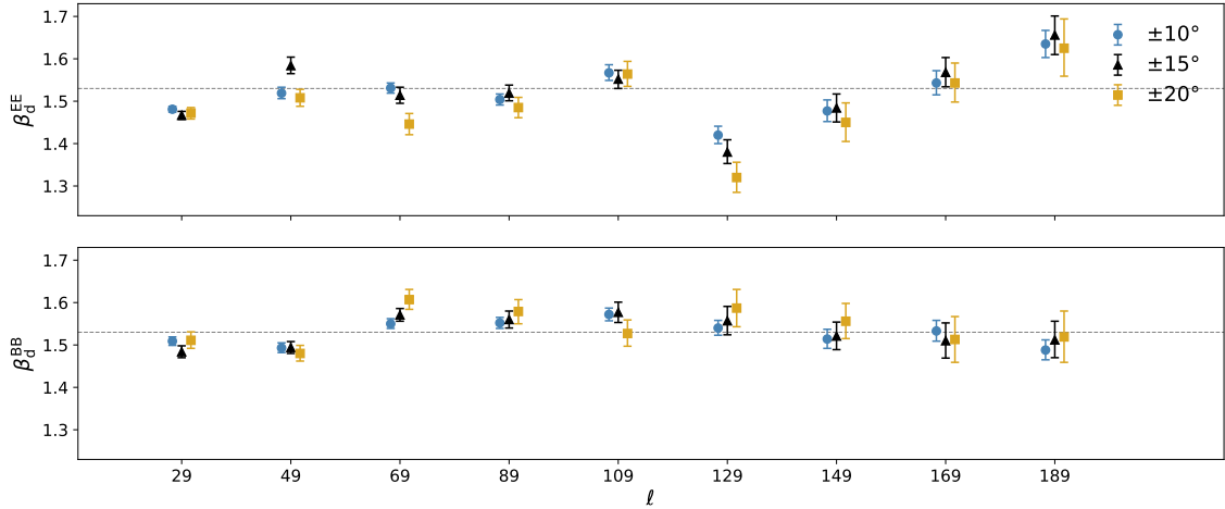
Figure 7: Dust spectral index \beta_d for E-modes (top panel) and B-modes (bottom panel), for the three Galactic cuts from the bin-to-bin analysis (Tables 2, 3 and 4) using the WM+Pl+QJ dataset. The dashed line marks the \beta_d = 1.53 value as a reference.
