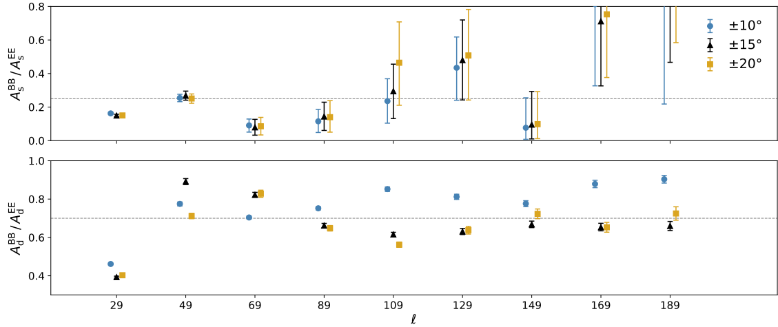
Figure 5: Synchrotron and dust B-to-E amplitude ratio A_s^{BB}/A_s^{EE} and A_d^{BB}/A_d^{EE} respectively, for the three Galactic cuts from the bin-to-bin analysis (Tables 2, 3 and 4) using the WM+Pl+QJ dataset. The dashed line marks the A_s^{BB}/A_s^{EE} = 0.25 and A_d^{BB}/A_d^{EE} = 0.70 values as a reference.
