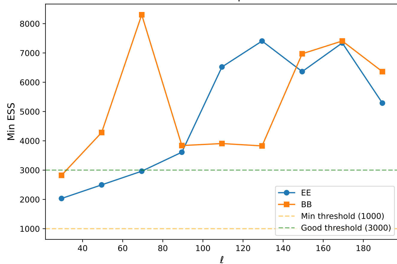
ESS Distribution
