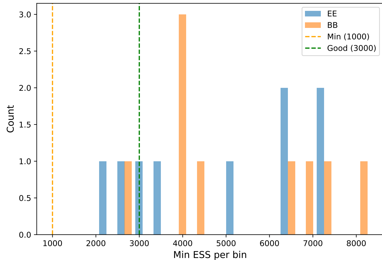
ESS Distribution
