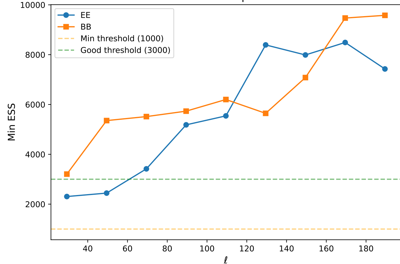
ESS Distribution
