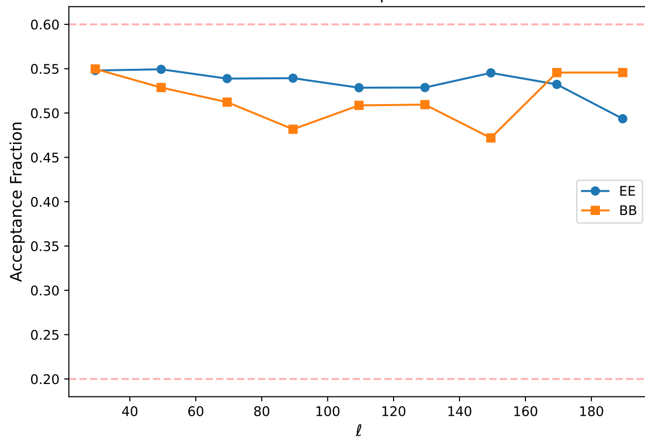
MCMC Acceptance
