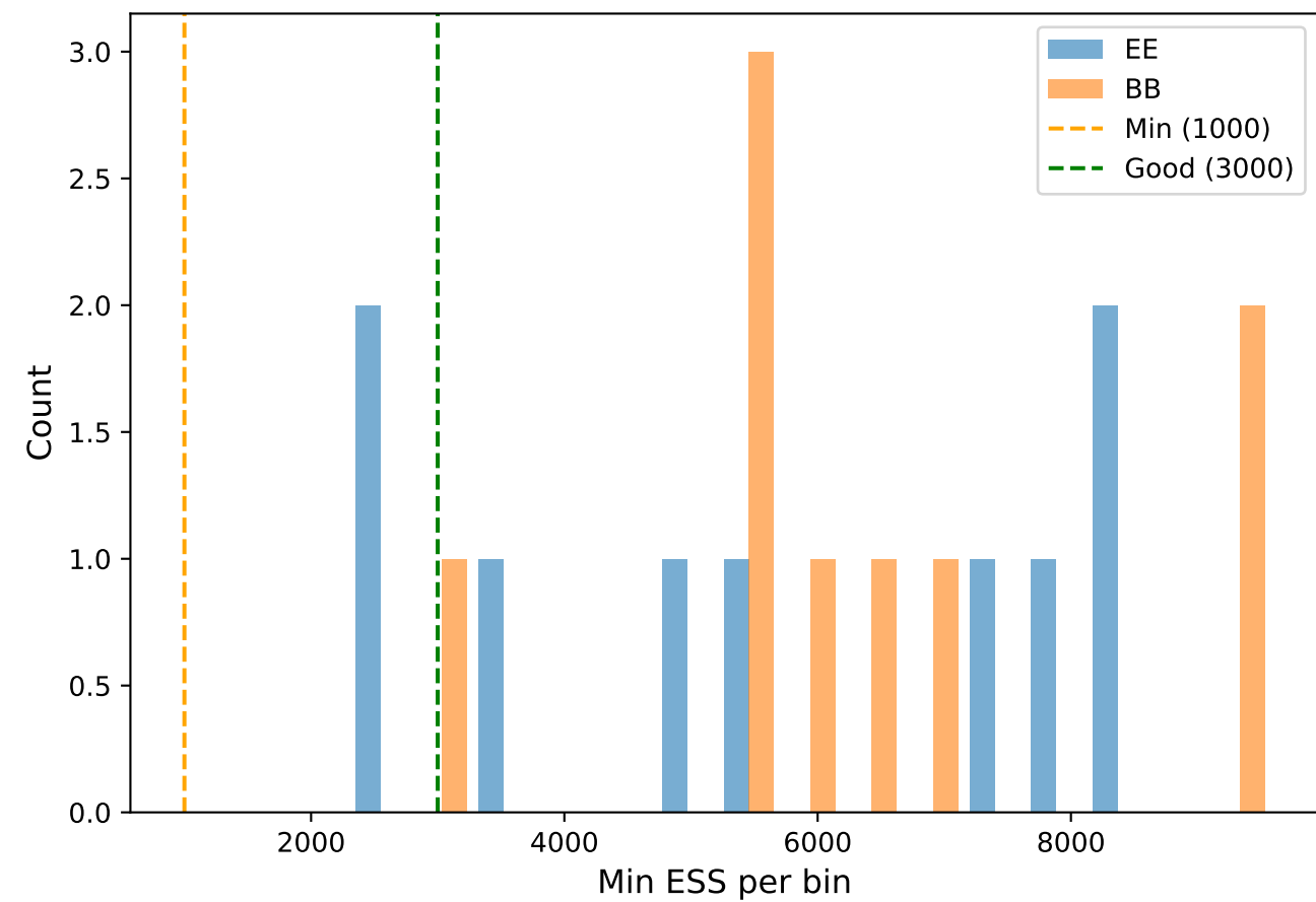
ESS Distribution
