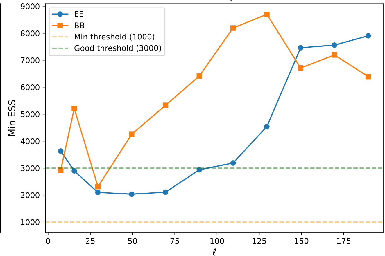
ESS Distribution
