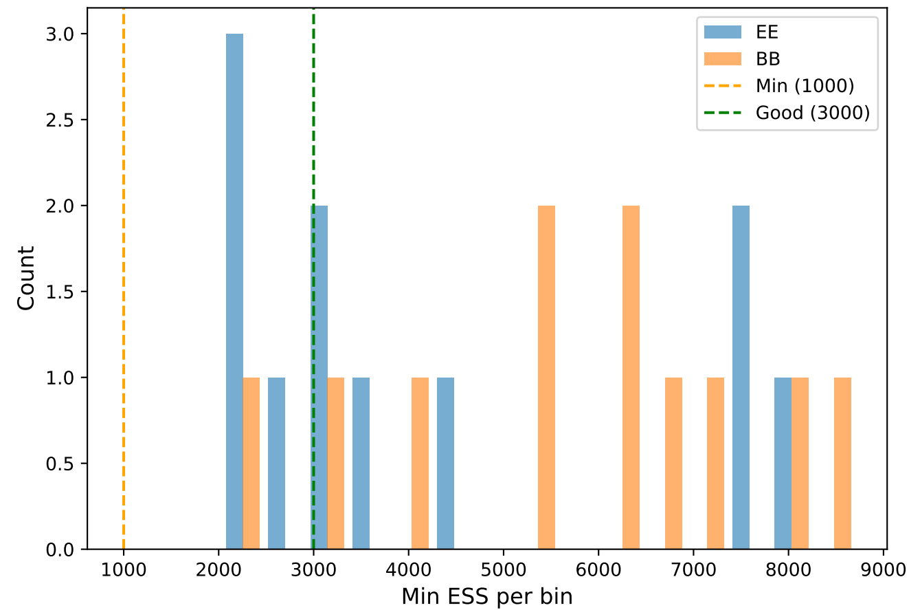
ESS Distribution
