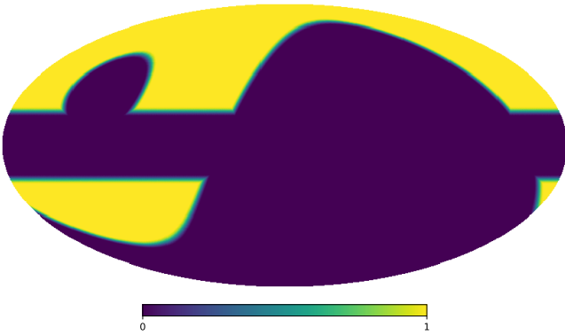
Figure 2: Analysis mask combining the QUIJOTE low-declination survey mask with a 15^\circ cut in galactic latitude.
