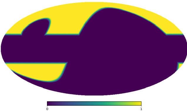
Figure 3: Analysis mask combining the QUIJOTE low-declination survey mask with a 20^\circ cut in galactic latitude.
