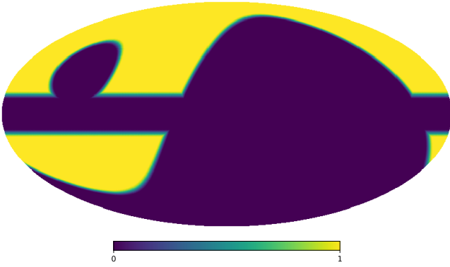
Figure 1: Analysis mask combining the QUIJOTE low-declination survey mask with a 10^\circ cut in galactic latitude.
