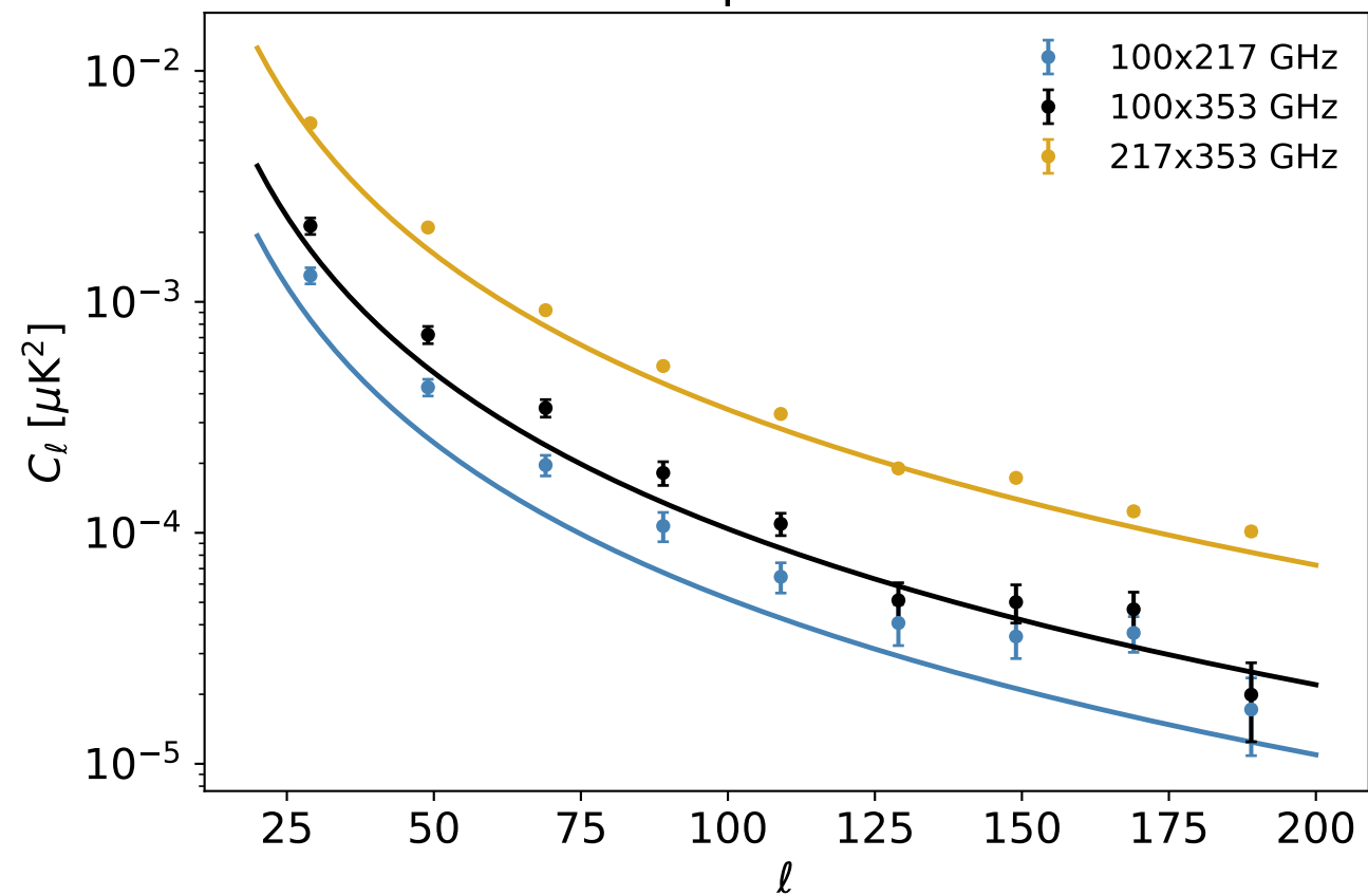
Cross-spectra — BB
