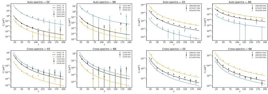
Figure 3: Same as Figure 2 but for the |b| > 15^\circ Galactic mask.
