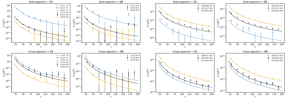
Figure 4: Same as Figure 2 but for the |b| > 20^\circ Galactic mask.
