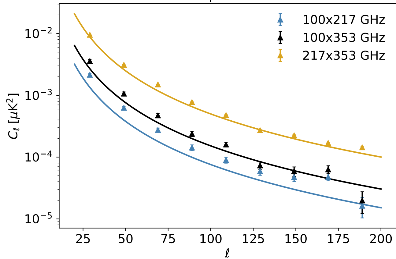
Cross-spectra — BB
