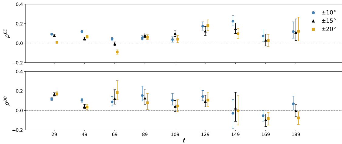
Figure 7: Synchrotron-dust spatial correlation \rho for E-modes (top panel) and B-modes (bottom panel), for the three Galactic cuts from the bin-to-bin analysis (Tables 2, 3 and 4) using the WM+P1+QJ dataset. The dashed line marks the \rho = 0 value as a reference.
