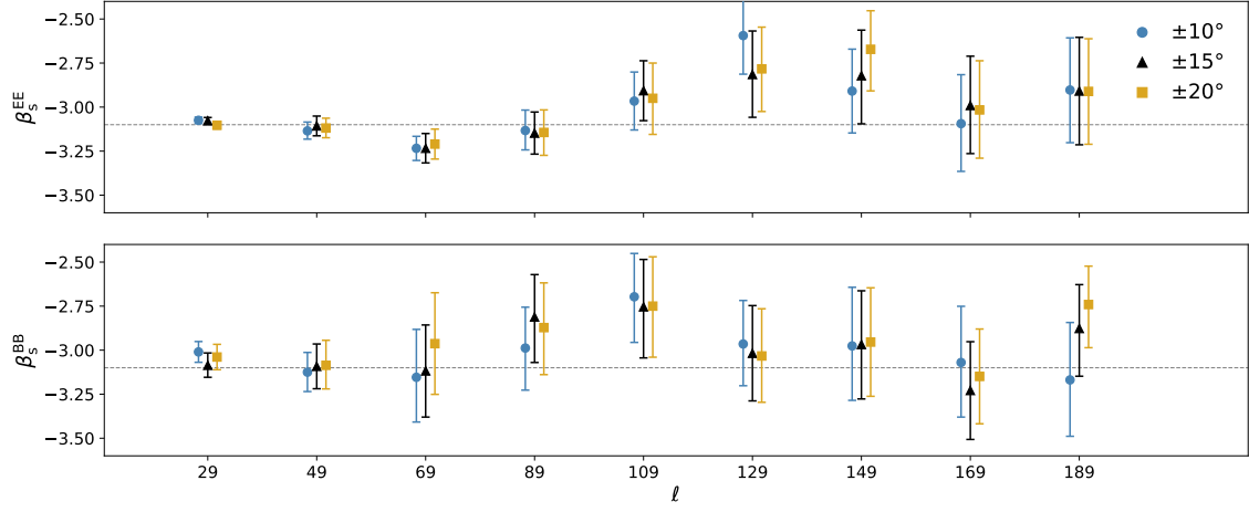
Figure 5: Synchrotron spectral index \beta_s for E-modes (top panel) and B-modes (bottom panel), for the three Galactic cuts from the bin-to-bin analysis (Tables 2, 3 and 4) using the WM+Pl+QJ dataset. The dashed line marks the \beta_s = -3.1 value as a reference.
