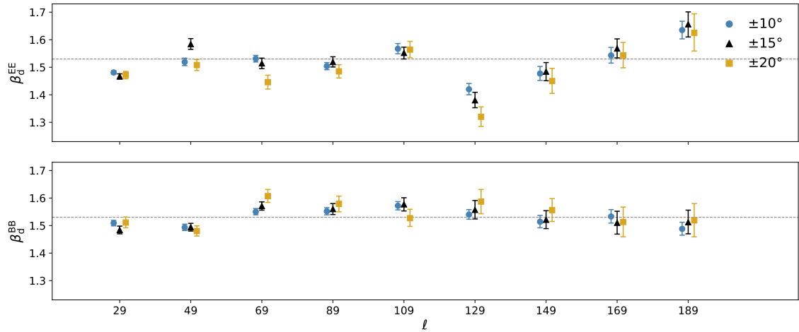
Figure 6: Dust spectral index \beta_d for E-modes (top panel) and B-modes (bottom panel), for the three Galactic cuts from the bin-to-bin analysis (Tables 2, 3 and 4) using the WM+Pl+QJ dataset. The dashed line marks the \beta_d = 1.53 value as a reference.
