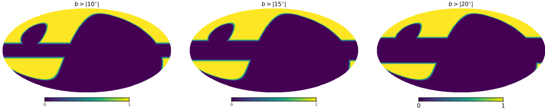
Figure 2: Analysis masks combining the QUIJOTE low-declination survey footprint with Galactic latitude cuts of |b| > 10^{\circ} (left), |b| > 15^{\circ} (middle), and |b| > 20^{\circ} (right), after C2 apodisation with a 5^{\circ} border.
