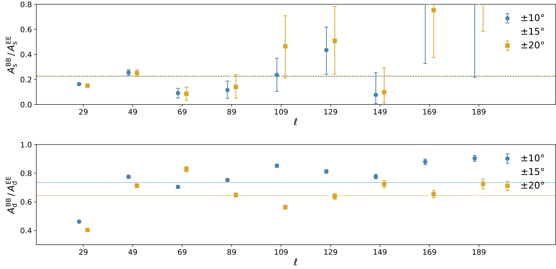
Figure 5: Synchrotron and dust B-to-E amplitude ratios A_s^{BB}/A_s^{EE} (top panel) and A_d^{BB}/A_d^{EE} (bottom panel), for the three Galactic cuts masks from the bin-to-bin analysis (Tables 2, 3 and 4) using the QJ+WP+Pl dataset. The dashed line marks the A_s^{BB}/A_s^{EE} = 0.25 and A_d^{BB}/A_d^{EE} = 0.70 values as a reference.
