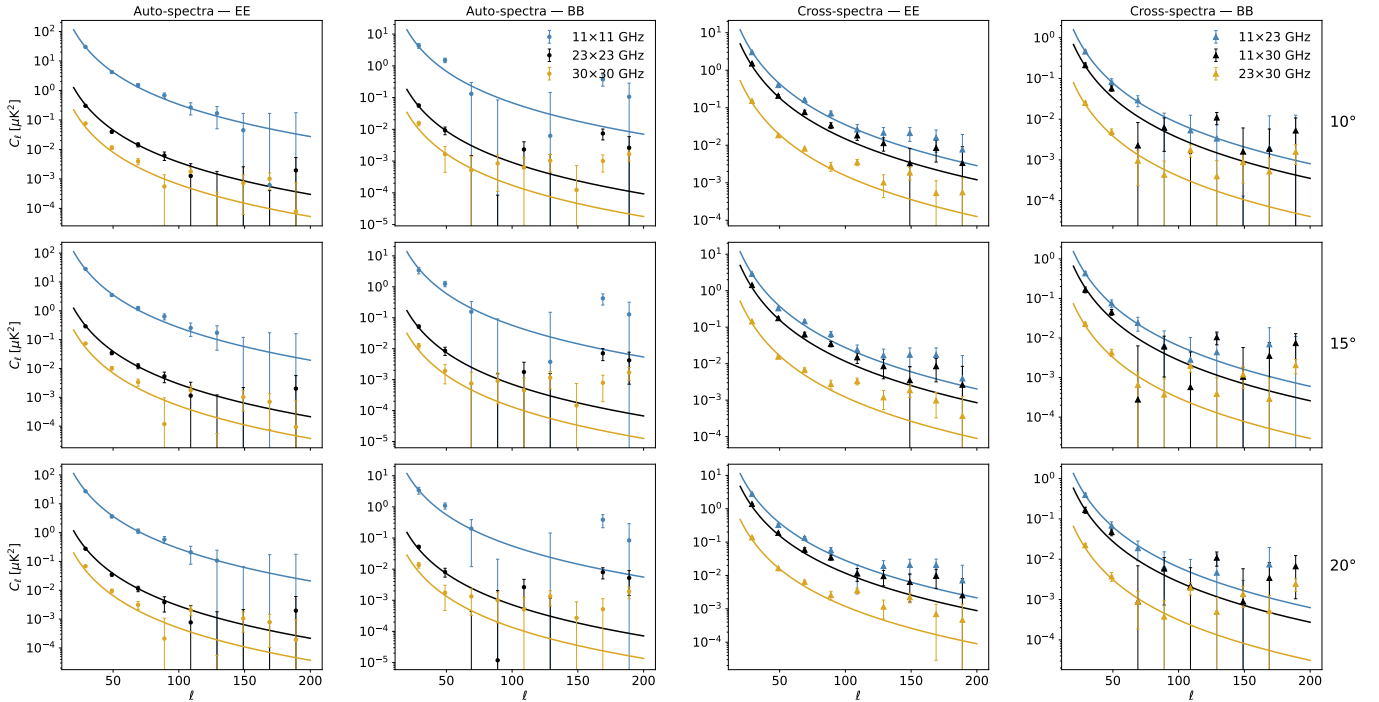
Figure 9: Measured auto- and cross-power spectra in the low-frequency bands (11, 23 and 30 GHz) for three Galactic masks. Each row corresponds to a mask (top to bottom: |b| > 10^\circ, 15^\circ, 20^\circ ) and the four columns show, from left to right, auto-spectra EE, auto-spectra BB, cross-spectra EE and cross-spectra BB. Markers are binned band powers C_\ell with 1\sigma uncertainties (circles for auto-spectra, and triangles for cross-spectra). Solid lines show the best-fit full model from Equation 16 using only cross data, and evaluated for each band pair.
